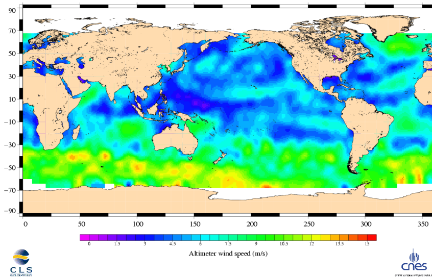
Jason-1 Cycle 133 16/08/2005 – 25/08/2005
