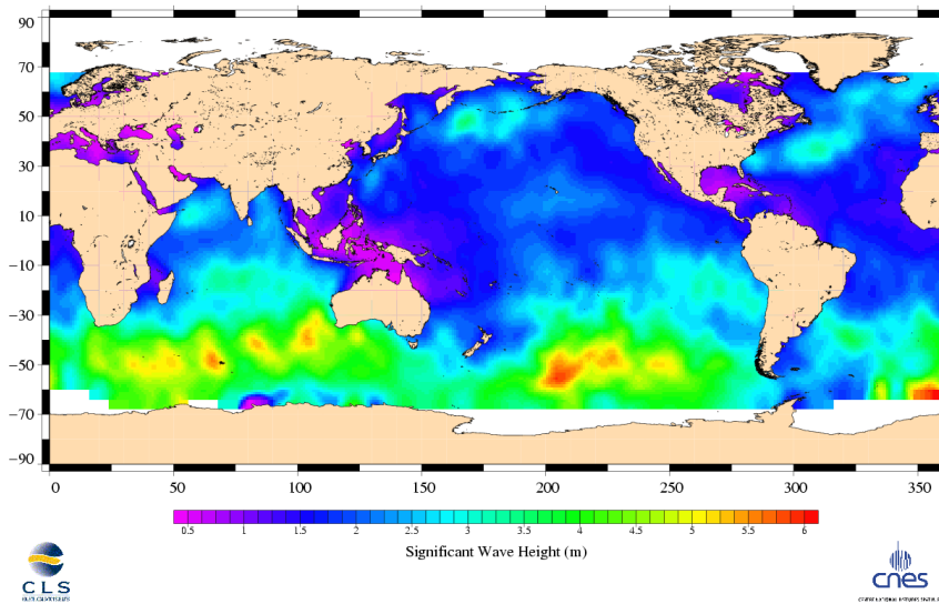
Jason-1 Cycle 135 04/09/2005 – 14/09/2005
