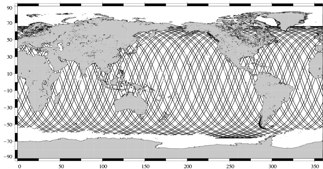
Valid data Jason-1 Cycle 136 (14/09/2005 / 20/09/2005)
