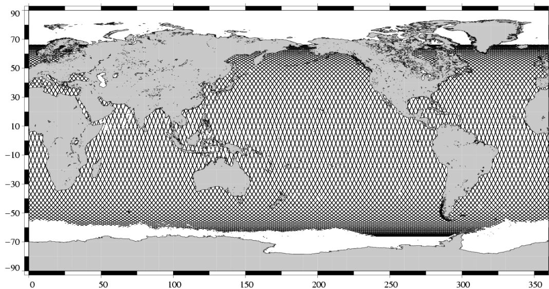
Valid data Jason-1 Cycle 140 (24/10/2005 / 03/11/2005)
