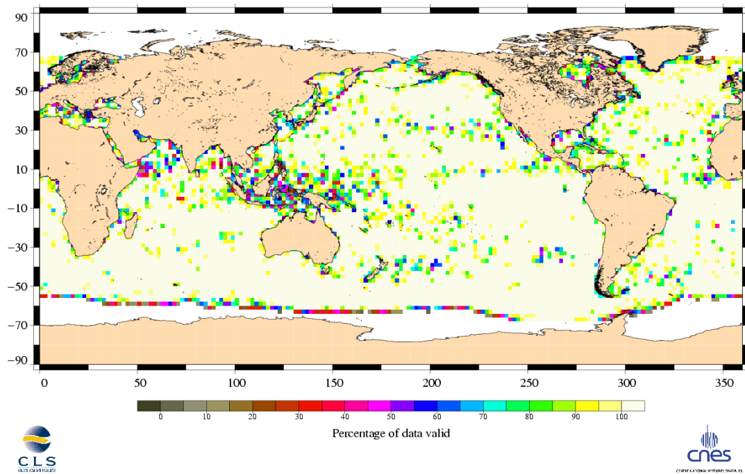
Percentage of valid data relative to the nominal pass Jason-1 Cycle 140 (24/10/2005 / 03/11/2005)
