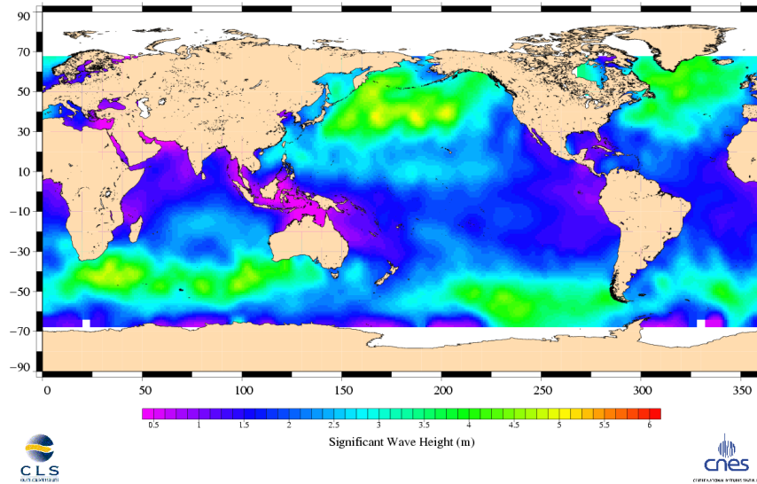
Jason-1 Cycle 144 03/12/2005 - 13/12/2005
