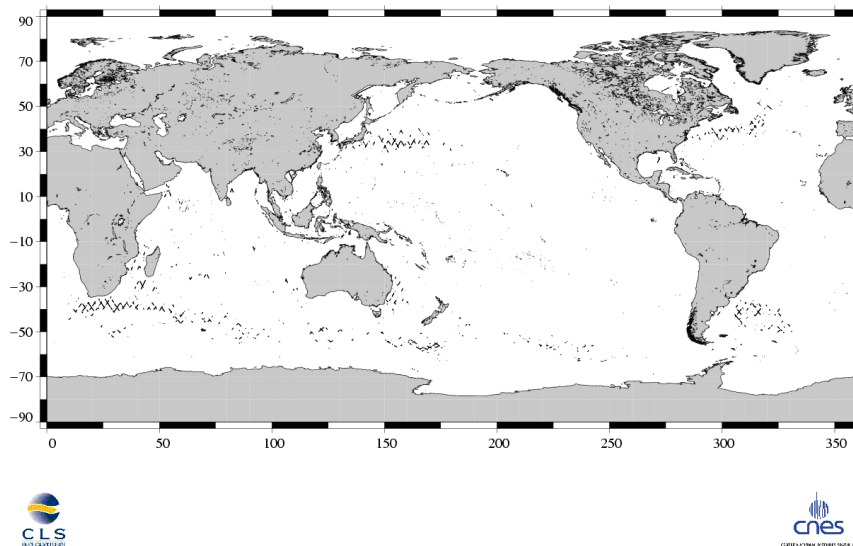
(SSH – MSS) differences greater than 30 cm Jason / Cycle 144
