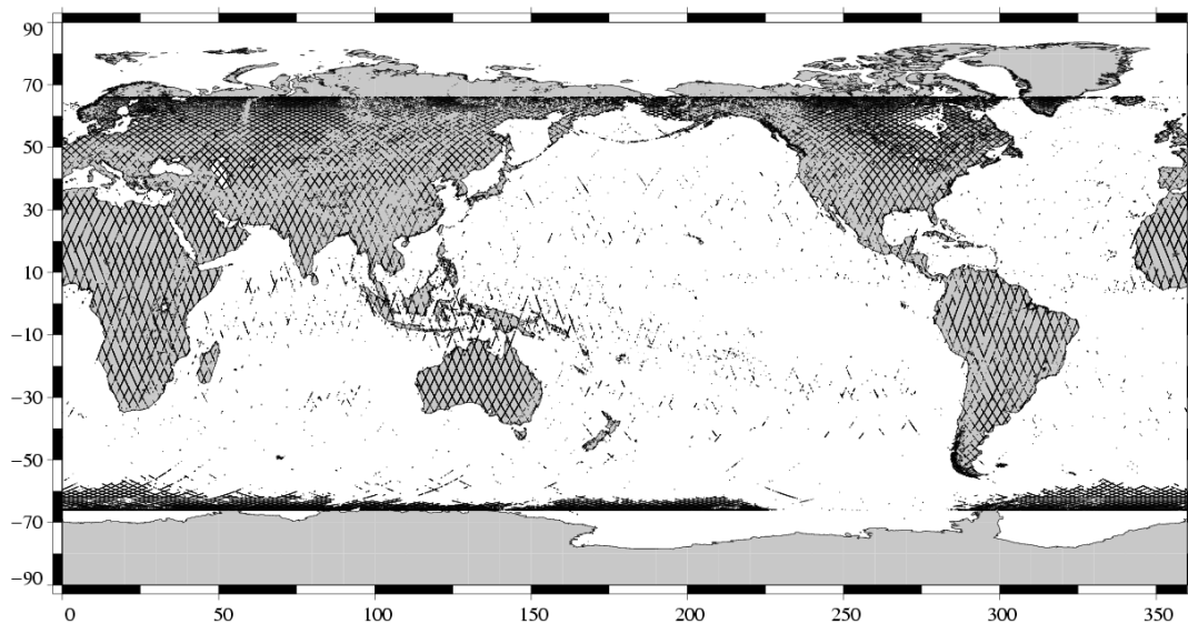
Edited measurements Jason-1 Cycle 144 (03/12/2005 / 13/12/2005)
