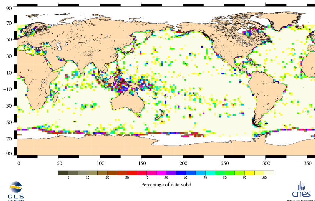
Percentage of valid data relative to the nominal pass Jason-1 Cycle 144 (03/12/2005 / 13/12/2005)
