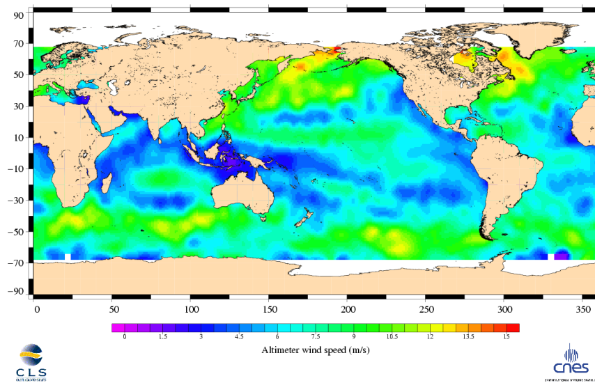
Jason-1 Cycle 144 03/12/2005 - 13/12/2005
