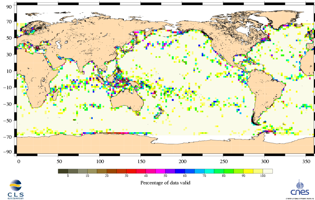
Percentage of valid data relative to the nominal pass Jason-1 Cycle 150 (31/01/2006 / 10/02/2006)
