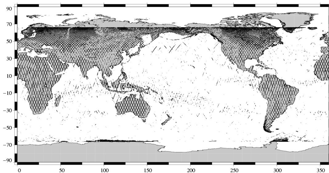
Edited measurements Jason-1 Cycle 150 (31/01/2006 / 10/02/2006)
