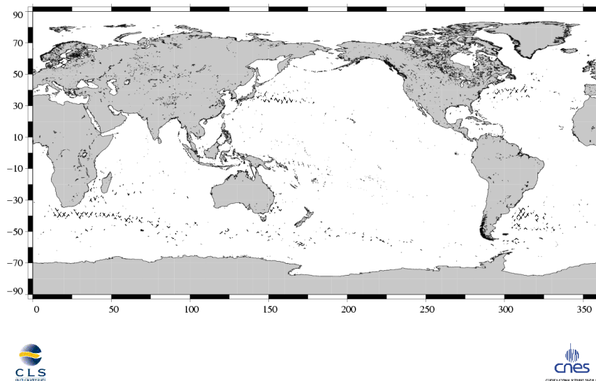
(SSH – MSS) differences greater than 30 cm Jason / Cycle 150
