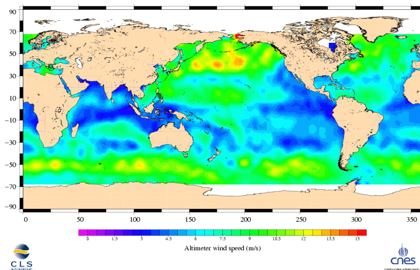
Jason-1 Cycle 150 31/01/2006 - 10/02/2006
