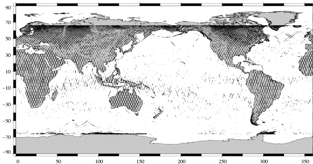
Edited measurements Jason-1 Cycle 151 (10/02/2006 / 20/02/2006)
