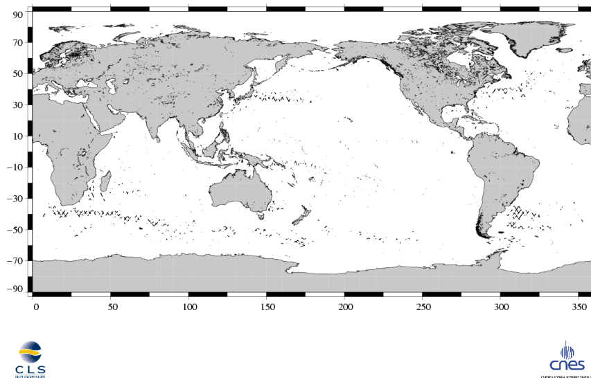
(SSH – MSS) differences greater than 30 cm Jason / Cycle 151
