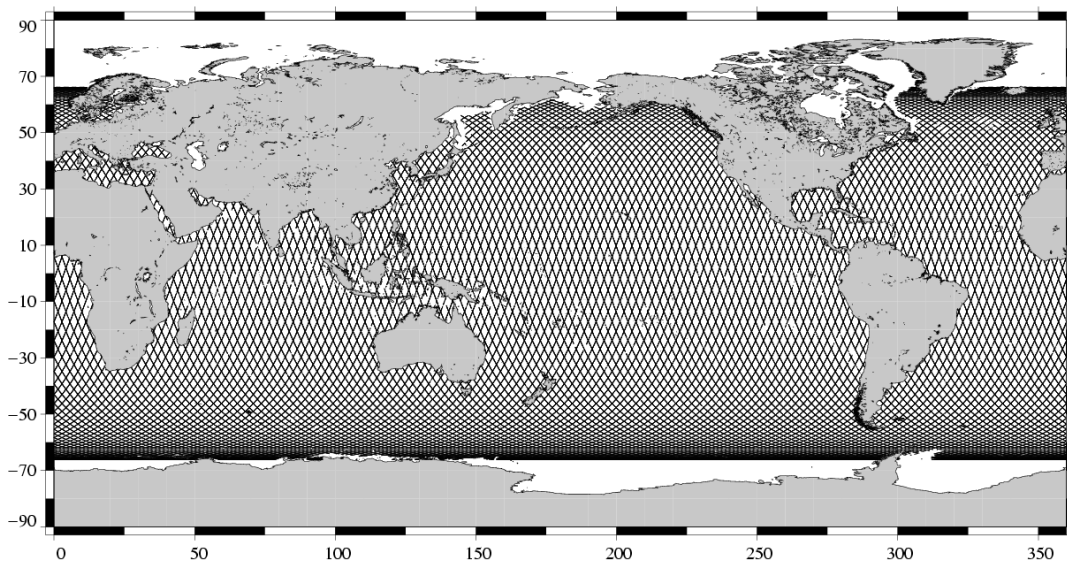
Valid data Jason-1 Cycle 151 (10/02/2006 / 20/02/2006)
