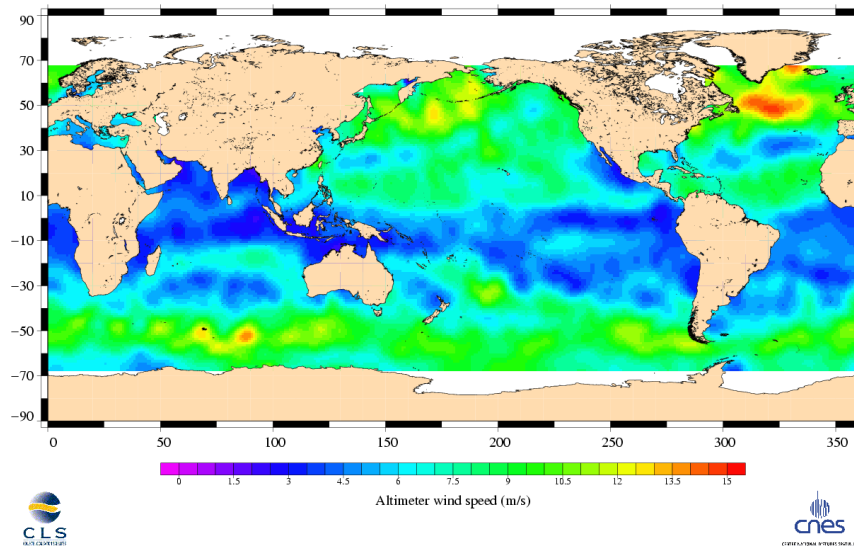
Jason-1 Cycle 151 10/02/2006 - 20/02/2006
