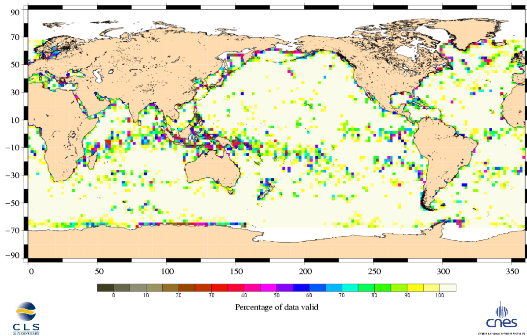
Percentage of valid data relative to the nominal pass Jason-1 Cycle 151 (10/02/2006 / 20/02/2006)
