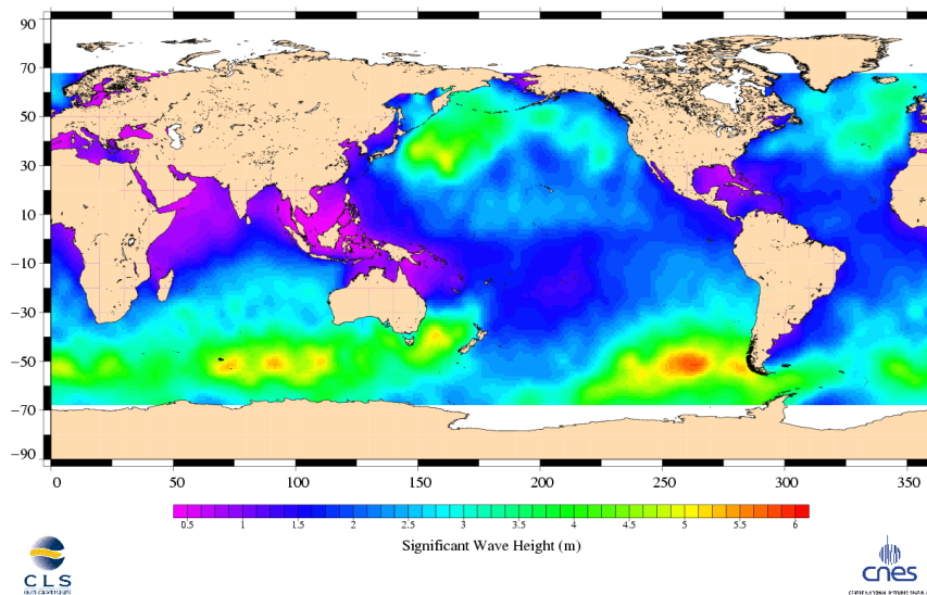
Jason-1 Cycle 156 01/04/2006 - 11/04/2006
