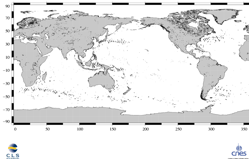
(SSH – MSS) differences greater than 30 cm Jason / Cycle 156
