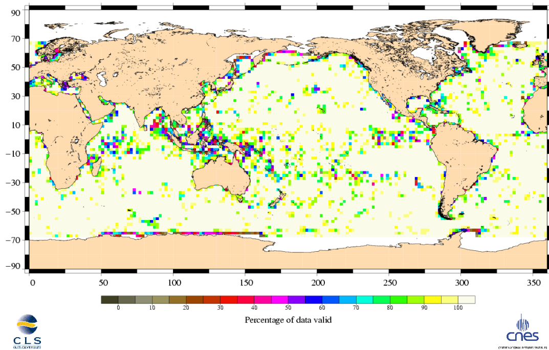
Percentage of valid data relative to the nominal pass Jason-1 Cycle 156 (01/04/2006 / 11/04/2006)
