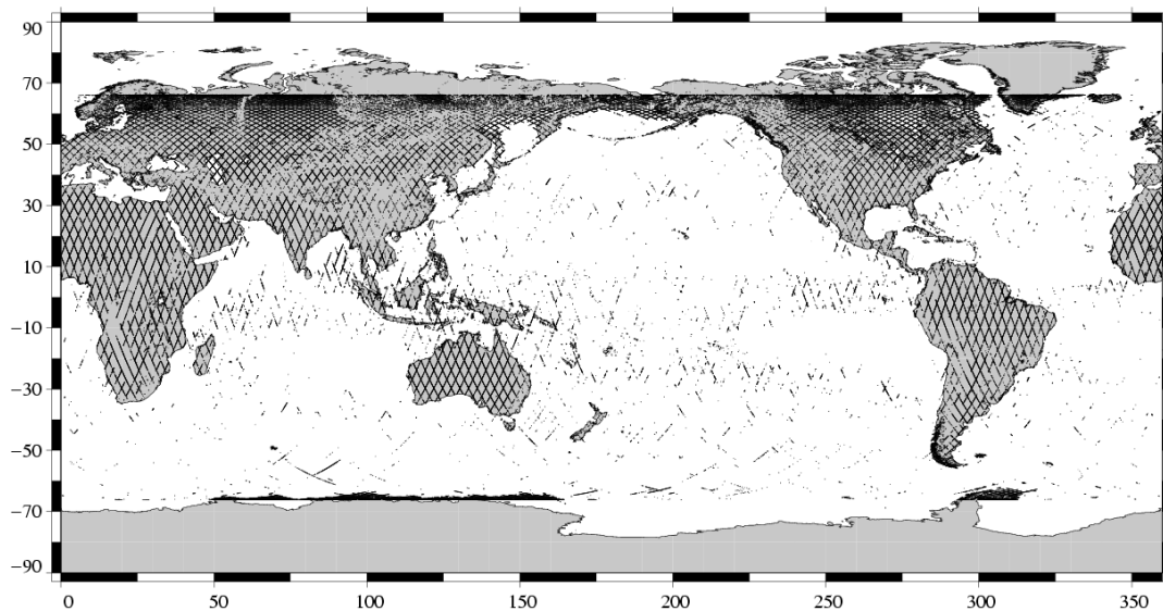
Edited measurements Jason-1 Cycle 156 (01/04/2006 / 11/04/2006)
