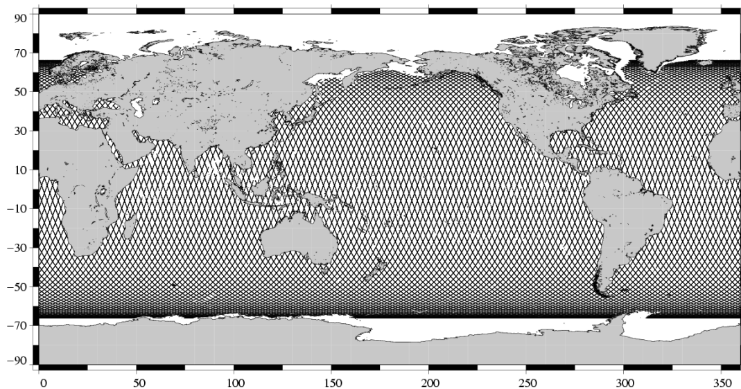
Valid data Jason-1 Cycle 156 (01/04/2006 / 11/04/2006)
