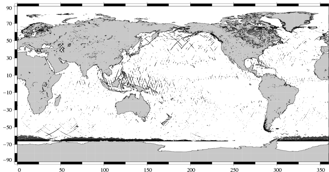
Edited measurements Jason-1 Cycle 162 (30/05/2006 / 09/06/2006)
