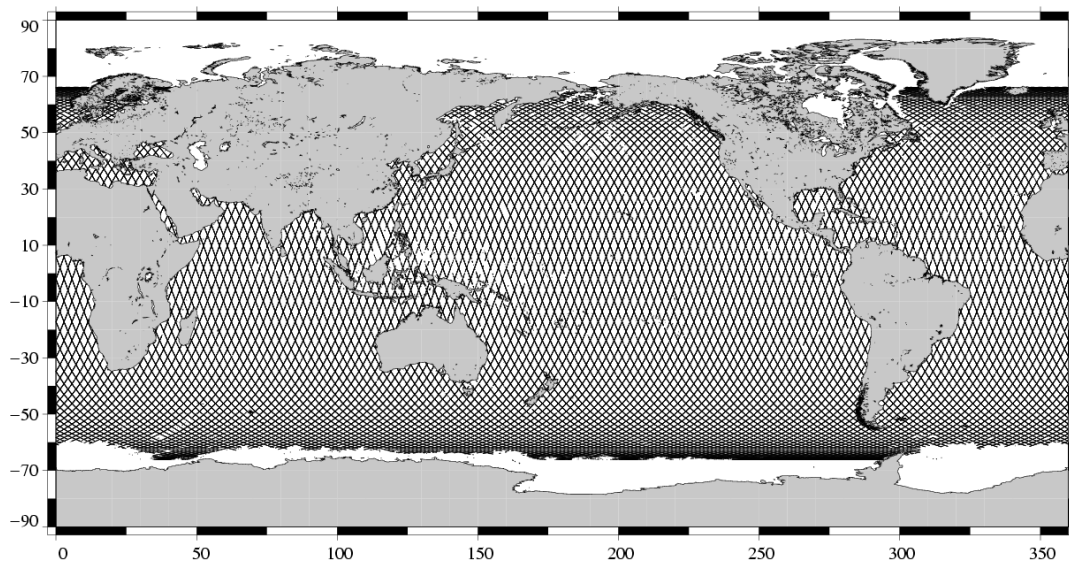
Valid data Jason-1 Cycle 162 (30/05/2006 / 09/06/2006)
