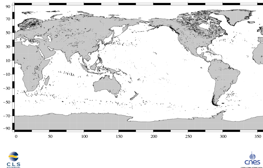
(SSH – MSS) differences greater than 30 cm Jason / Cycle 179
