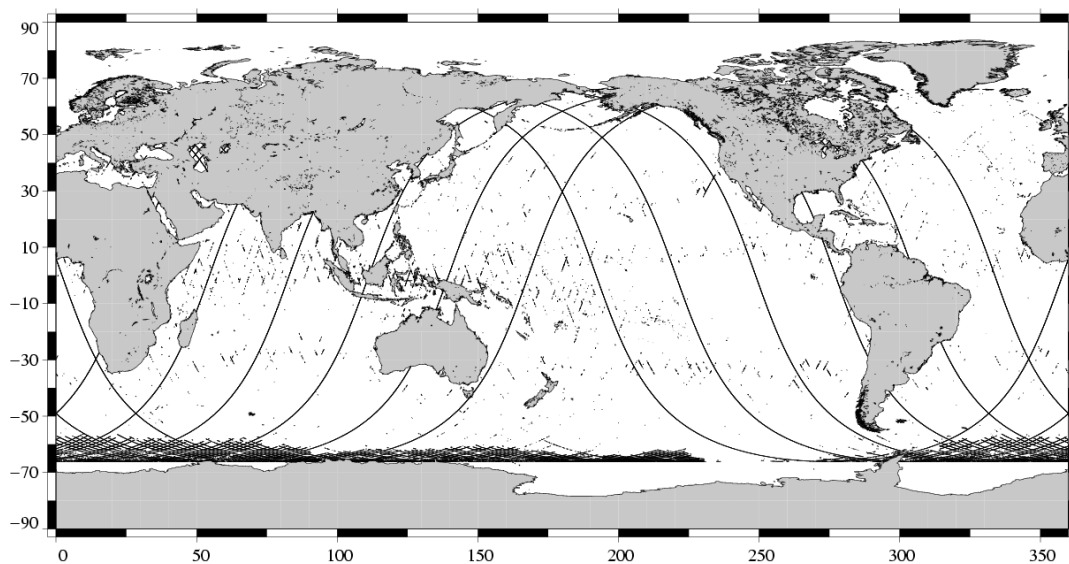
Edited measurements Jason-1 Cycle 179 (16/11/2006 / 25/11/2006)
