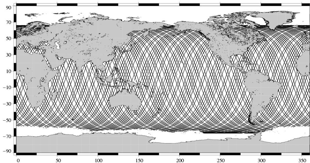
Valid data Jason-1 Cycle 179 (16/11/2006 / 25/11/2006)
