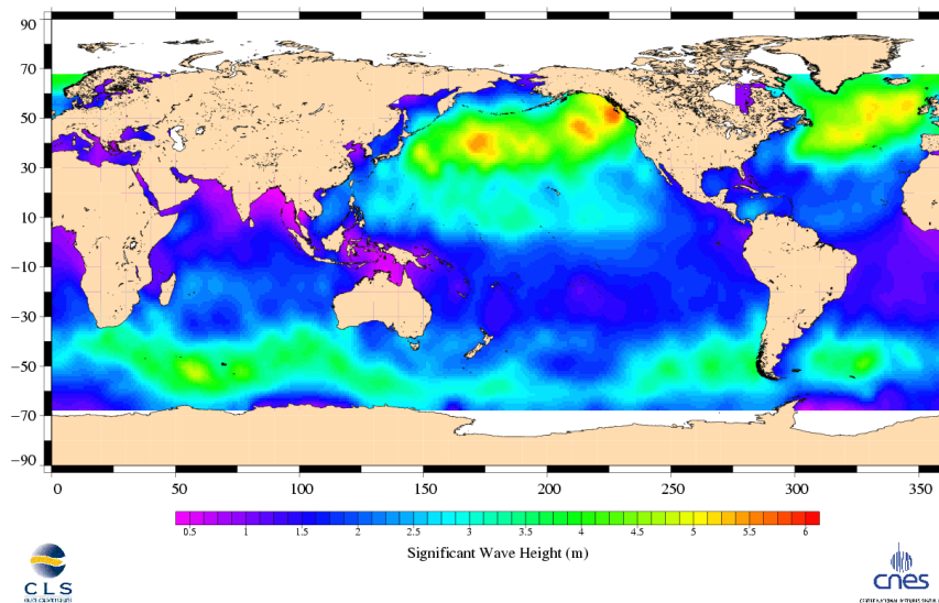
Jason-1 Cycle 183 24/12/2006 - 03/01/2007
