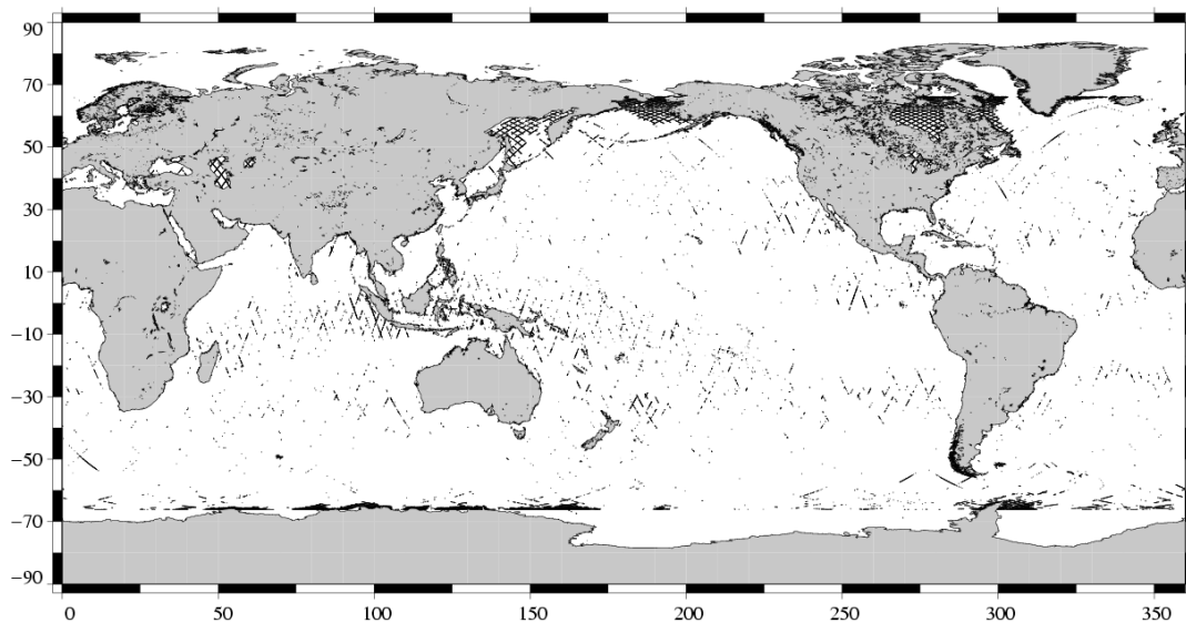
Edited measurements Jason-1 Cycle 186 (23/01/2007 / 02/02/2007)
