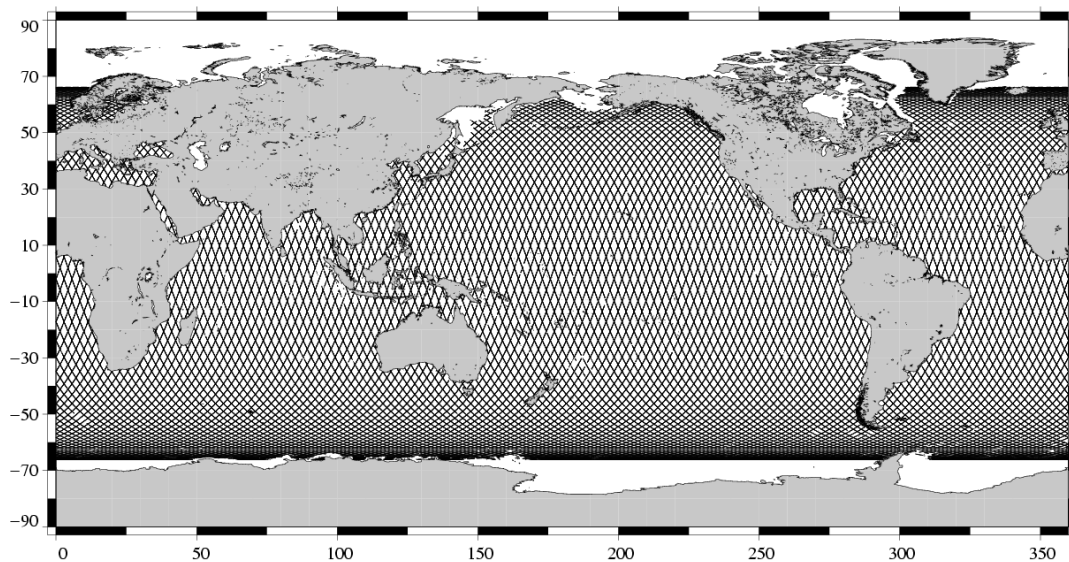
Valid data Jason-1 Cycle 186 (23/01/2007 / 02/02/2007)
