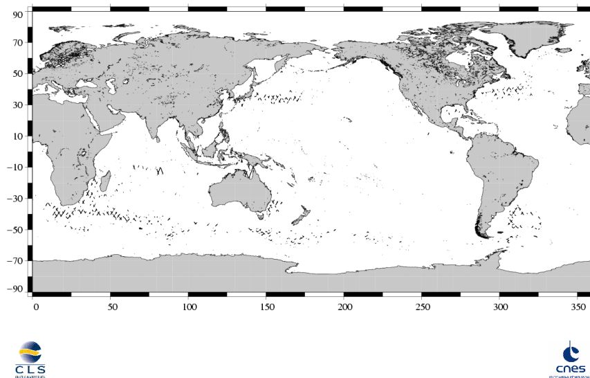
(SSH – MSS) differences greater than 30 cm Jason / Cycle 186
