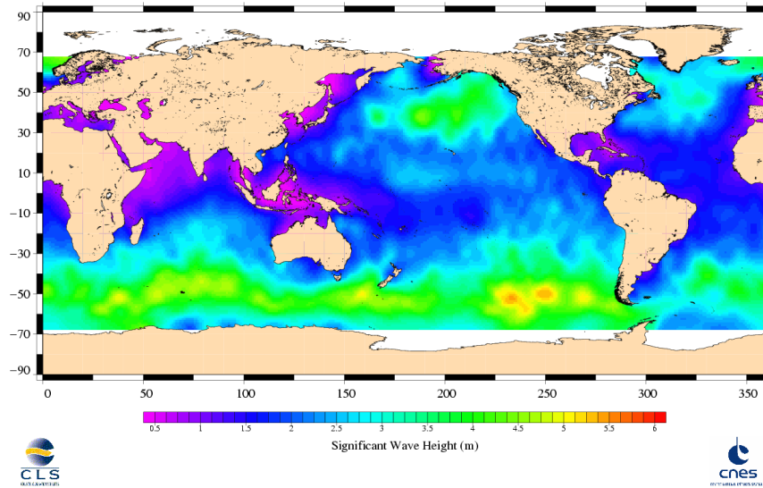
Jason-1 Cycle 193 03/04/2007 - 12/04/2007
