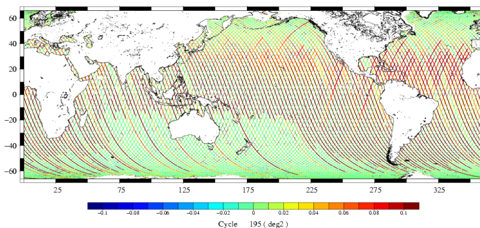
ATT_FO_CARRE [deg 2 ] J1 cycle 195
