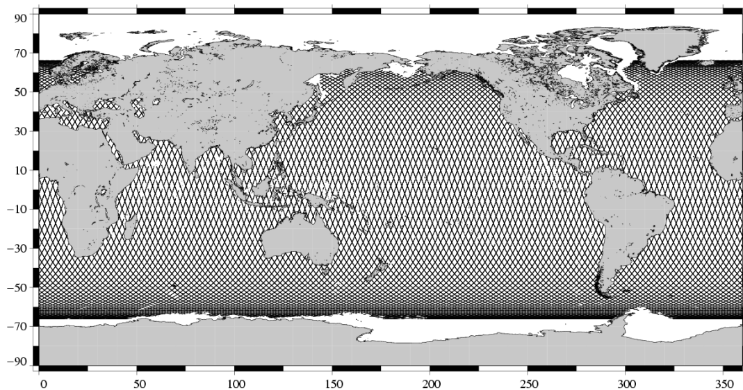
Valid data Jason-1 Cycle 195 (22/04/2007 / 02/05/2007)
