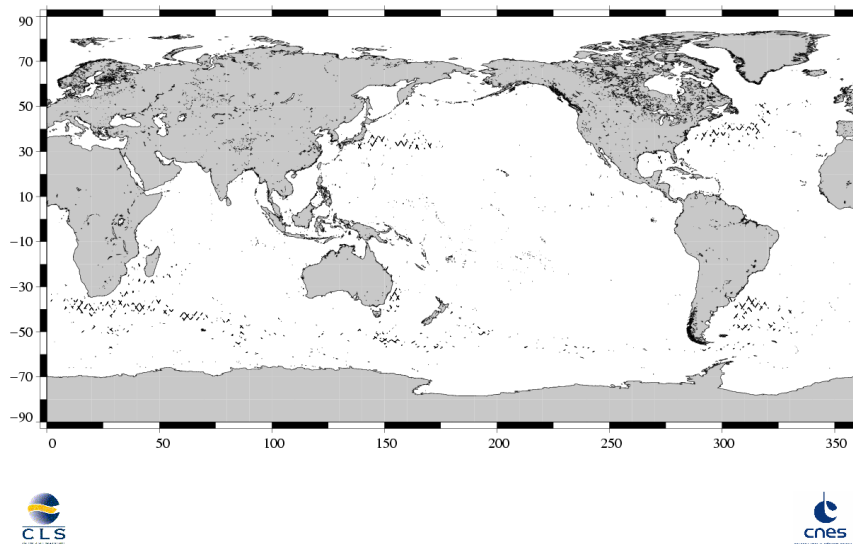
(SSH – MSS) differences greater than 30 cm Jason / Cycle 195
