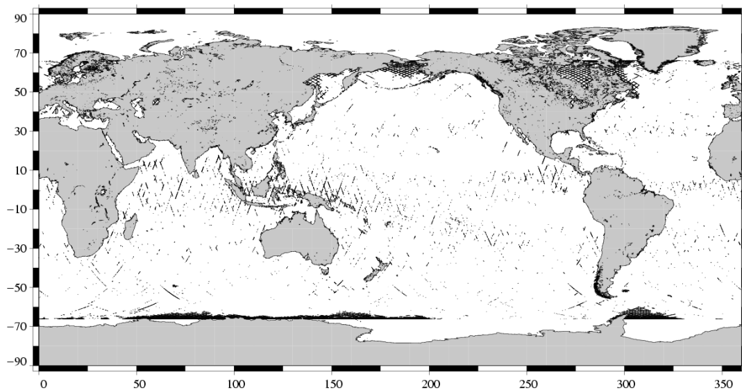
Edited measurements Jason-1 Cycle 195 (22/04/2007 / 02/05/2007)
