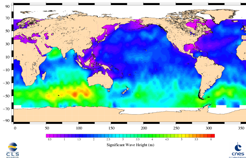
Jason-1 Cycle 202 01/07/2007 - 11/07/2007
