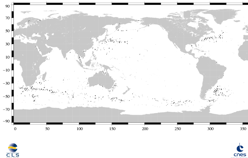
(SSH - MSS) differences greater than 30 cm Jason / Cycle 202
