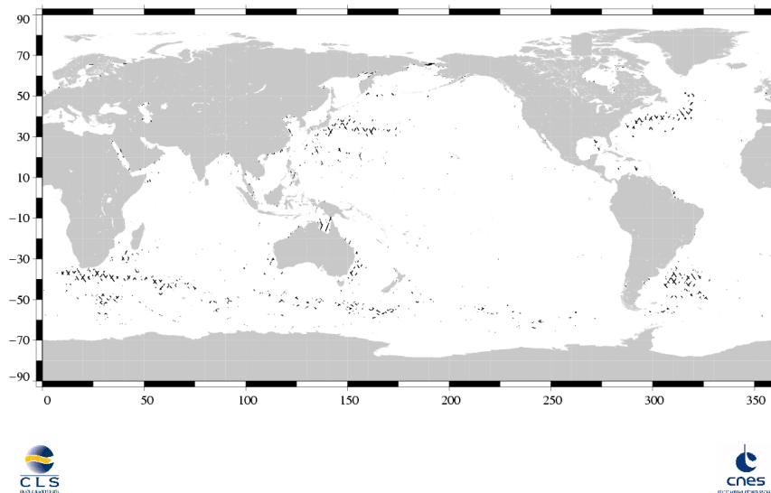
(SSH – MSS) differences greater than 30 cm Jason / Cycle 203
