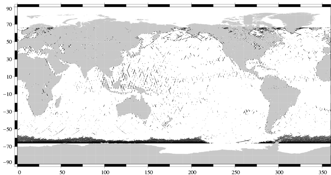
Edited measurements Jason-1 Cycle 203 (11/07/2007 / 21/07/2007)
