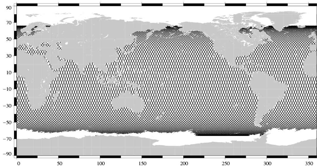
Valid data Jason-1 Cycle 203 (11/07/2007 / 21/07/2007)
