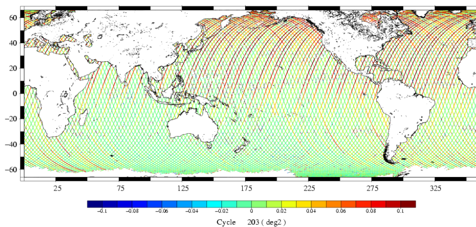
ATT_FO_CARRE [deg 2 ] J1 cycle 203
