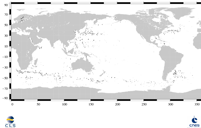
(SSH – MSS) differences greater than 30 cm Jason / Cycle 205
