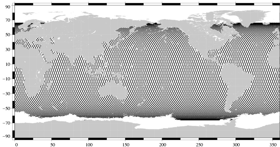
Valid data Jason-1 Cycle 205 (31/07/2007 / 09/08/2007)
