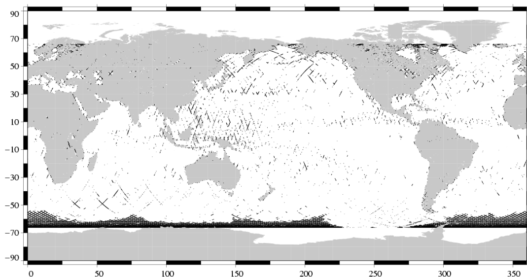
Edited measurements Jason-1 Cycle 205 (31/07/2007 / 09/08/2007)
