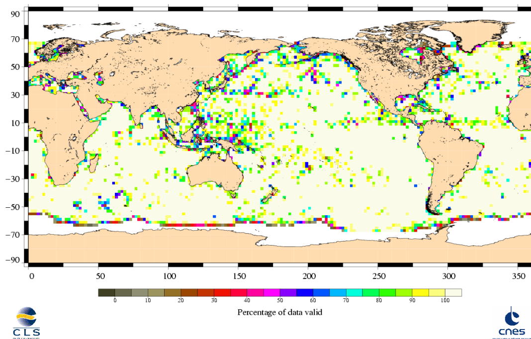
Percentage of valid data relative to the nominal pass Jason-1 Cycle 205 (31/07/2007 / 09/08/2007)
