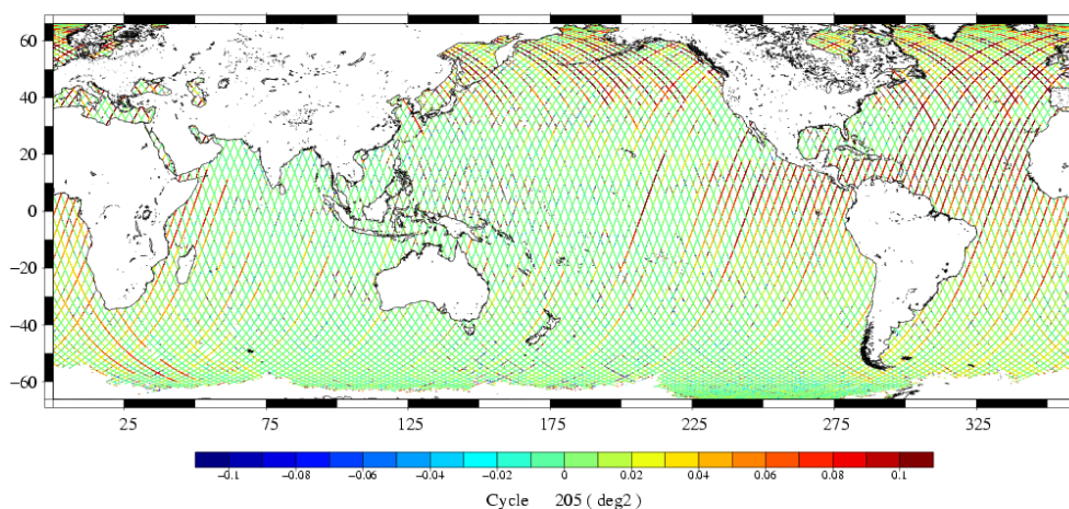
ATT_FO_CARRE [deg 2 ] J1 cycle 205
