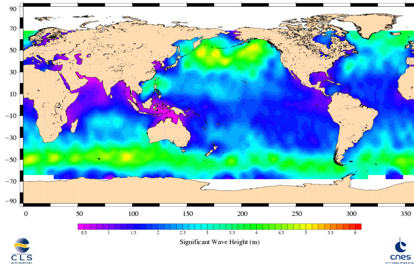
Jason-1 Cycle 216 17/11/2007 - 26/11/2007
