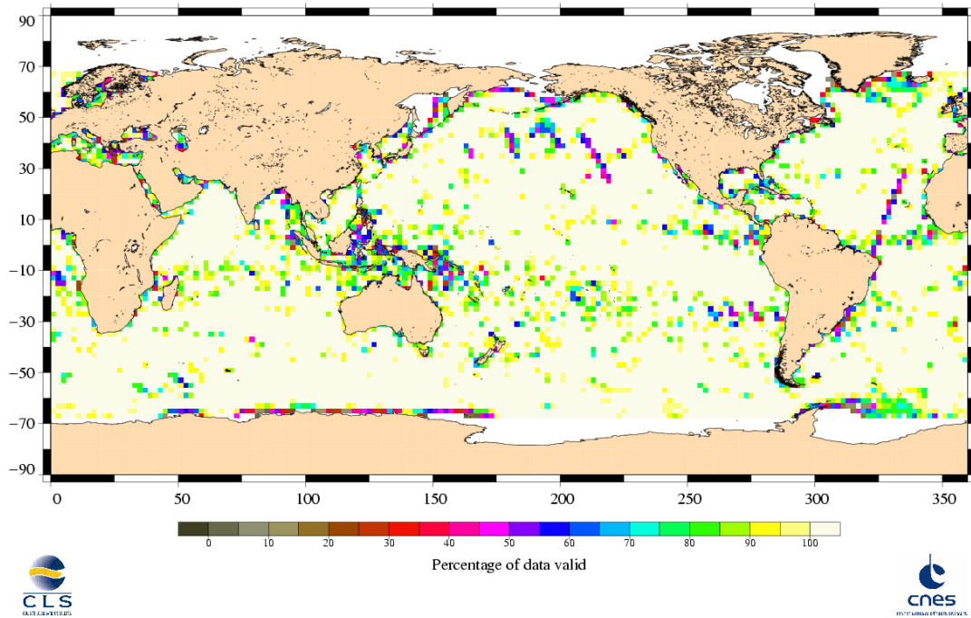
Percentage of valid data relative to the nominal pass Jason-1 Cycle 224 (04/02/2008 / 14/02/2008)
