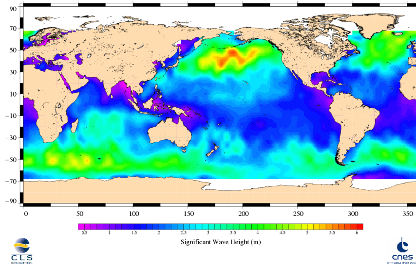
Jason-1 Cycle 224 04/02/2008 - 14/02/2008
