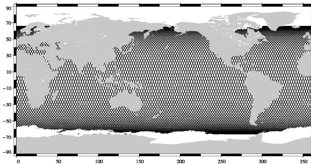
Valid data Jason-1 Cycle 253 (17/11/2008 / 27/11/2008)
