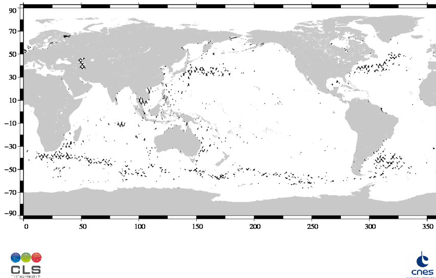
(SSH - MSS) differences greater than 30 cm Jason / Cycle 253
