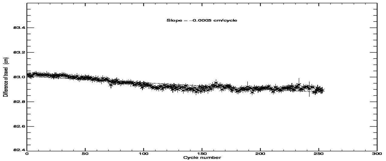
POSEIDON2 – Cycle 253 Difference of travel between E and R lines of the PTR in C band
