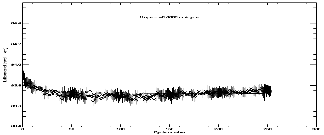
POSEIDON2 – Cycle 253 Difference of travel between E and R lines of the PTR in C band
