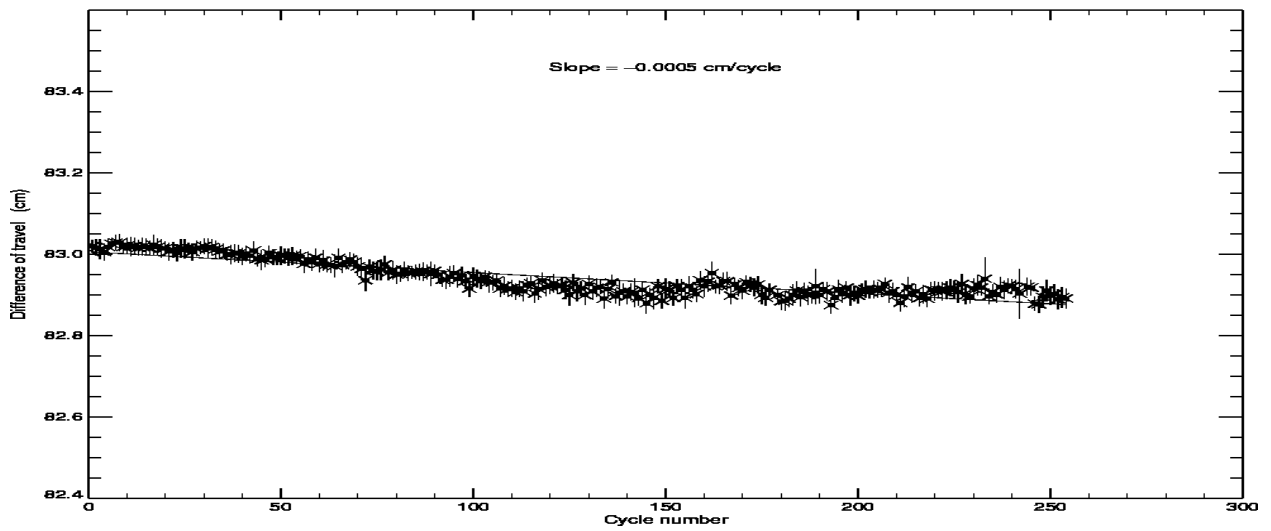
POSEIDON2 – Cycle 254 Difference of travel between E and R lines of the PTR in C band
