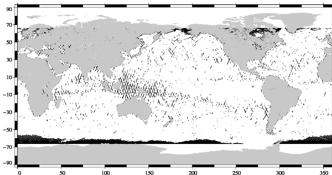
Edited measurements Jason-1 Cycle 254 (27/11/2008 / 07/12/2008)
