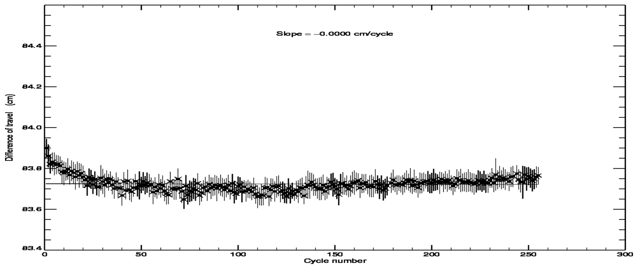
POSEIDON2 – Cycle 255 Difference of travel between E and R lines of the PTR in C band
