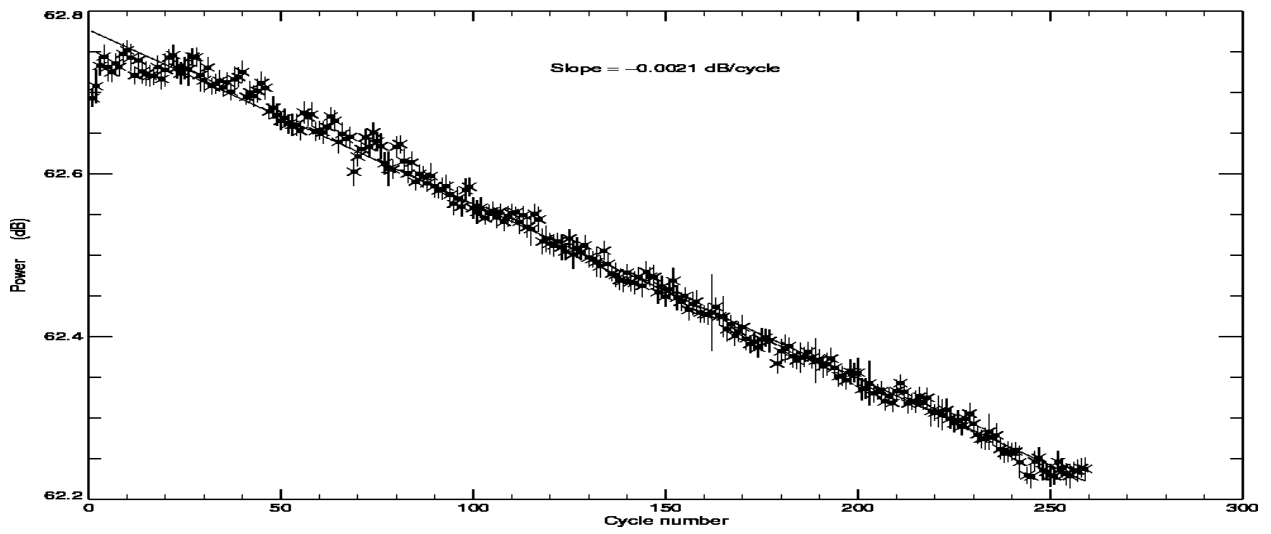
POSEIDON2 – Cycle 259 Total power of the PTR in C band
