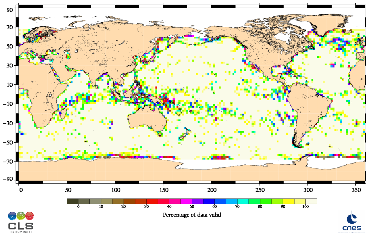
Percentage of valid data relative to the nominal pass Jason-1 Cycle 259 (16/01/2009 / 26/01/2009)
