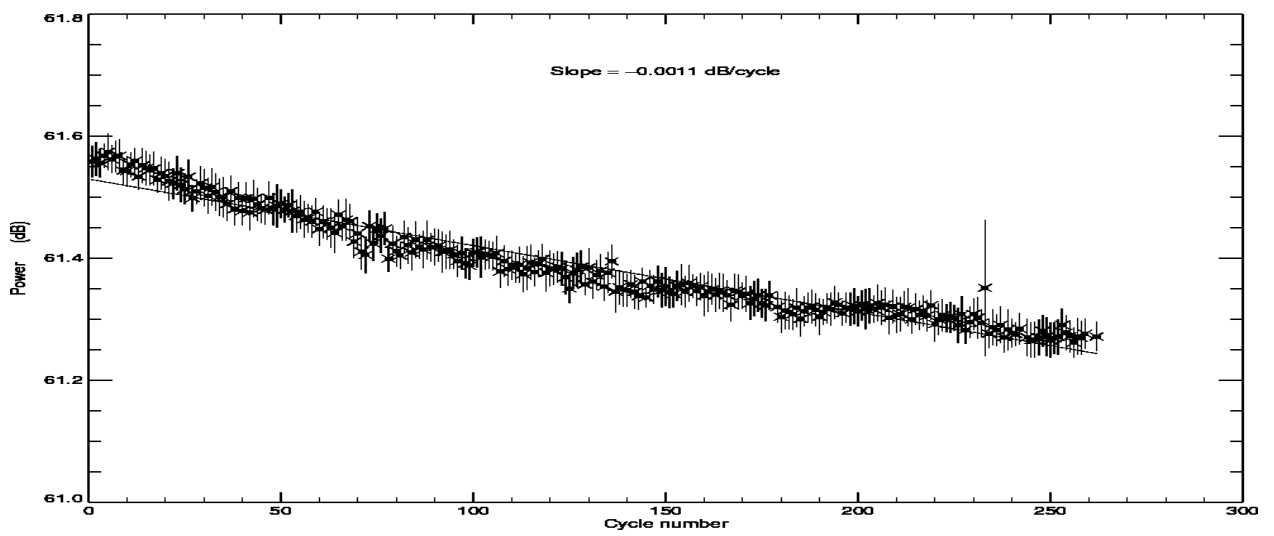
POSEIDON2 – Cycle 262 Total power of the PTR in C band
