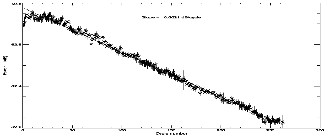
POSEIDON2 – Cycle 263 Total power of the PTR in C band
