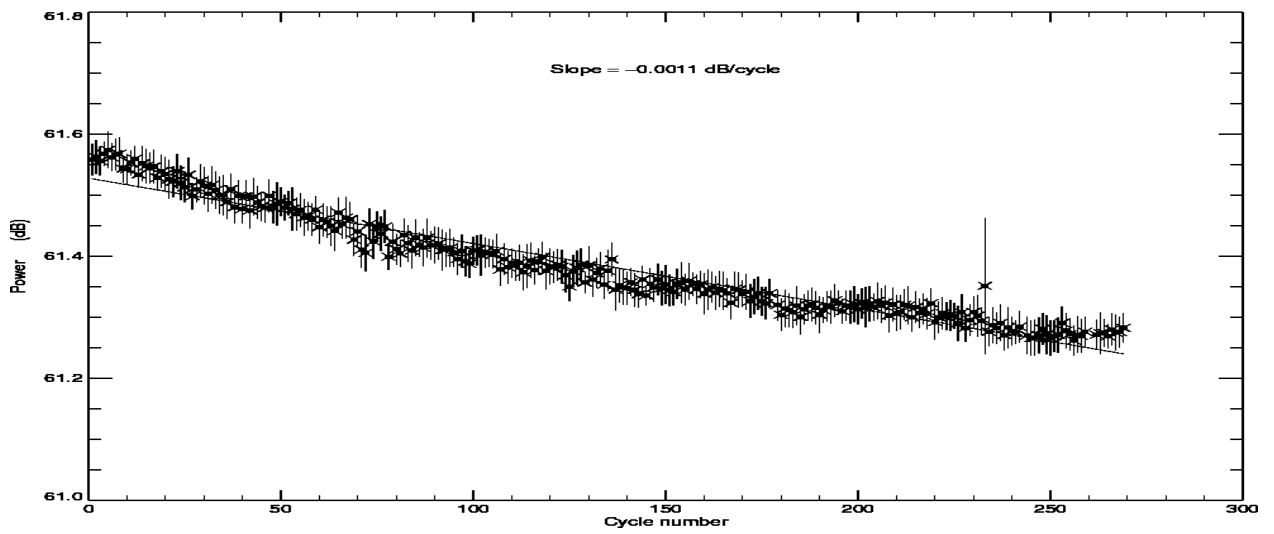
POSEIDON2 – Cycle 269 Total power of the PTR in C band
