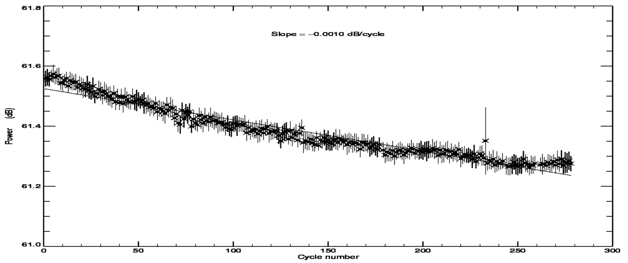
POSEIDON2 – Cycle 278 Total power of the PTR in C band
