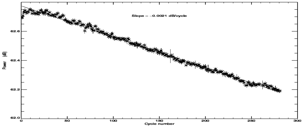
POSEIDON2 – Cycle 281 Total power of the PTR in C band
