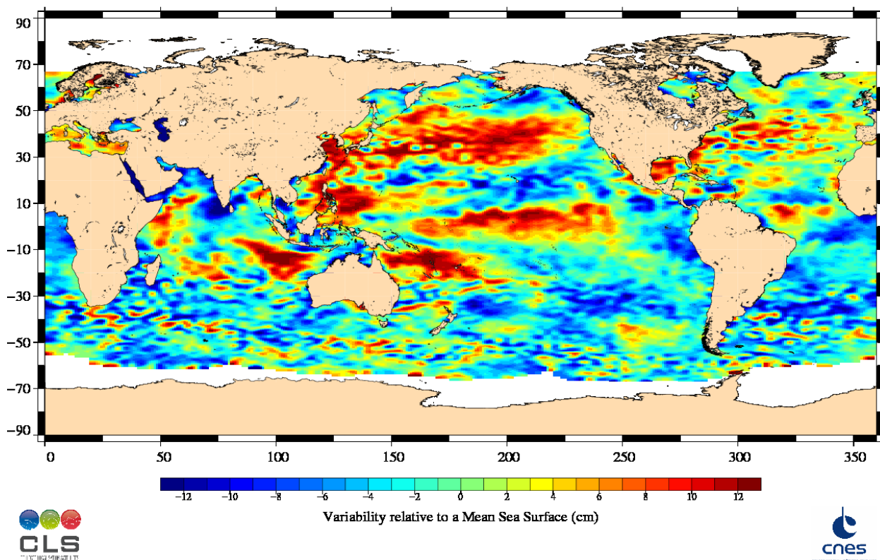
Jason-1 Cycle 282 27/08/2009 – 06/09/2009
