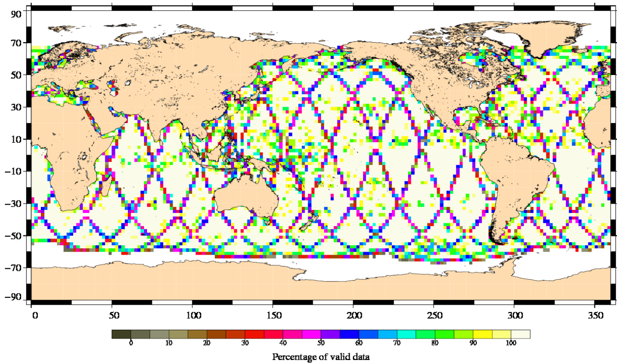
Percentage of valid data relative to the nominal pass Jason-1 Cycle 283 (06/09/2009 / 15/09/2009)
