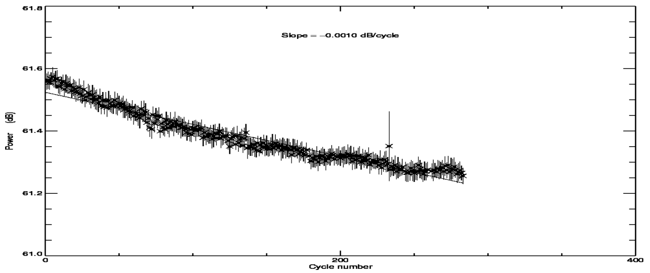
POSEIDON2 – Cycle 283 Total power of the PTR in C band
