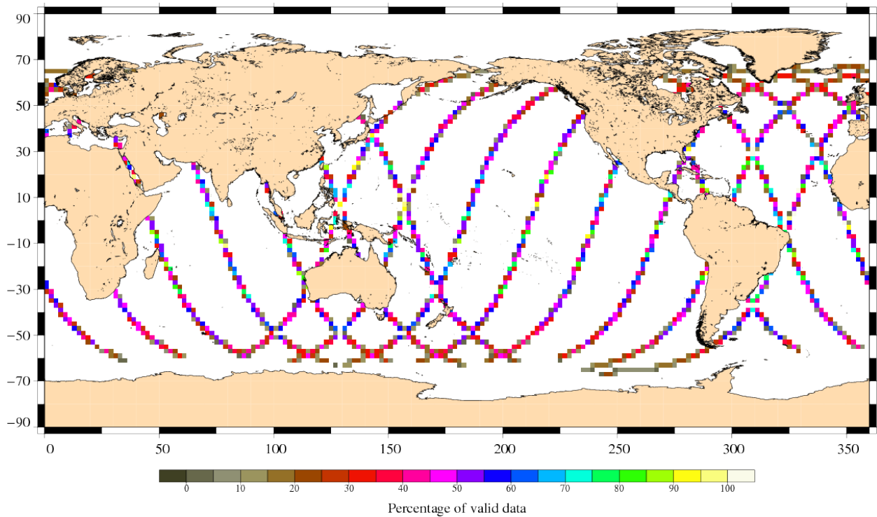
Percentage of valid data relative to the nominal pass Jason-1 Cycle 284 (25/09/2009 / 26/09/2009)
