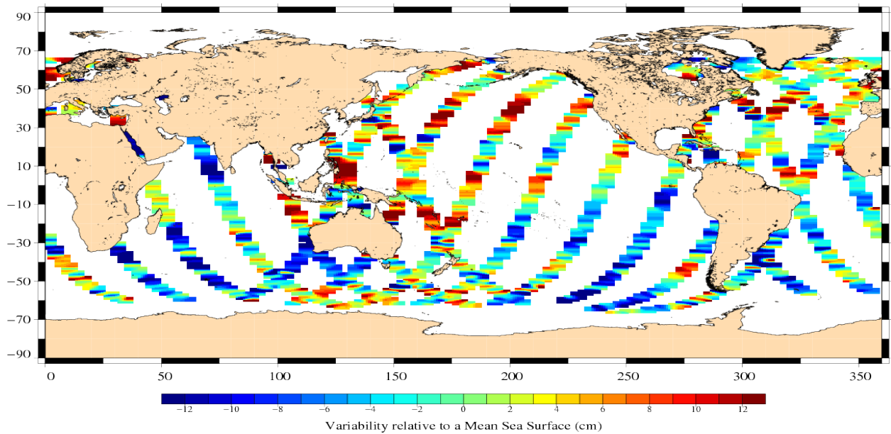
Jason-1 Cycle 284 25/09/2009 – 26/09/2009
