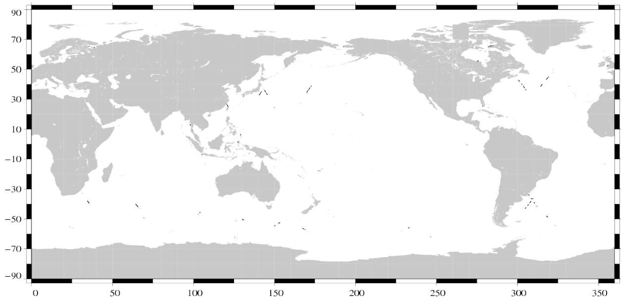
Valid data: (SSH – MSS) differences greater than 30 cm Jason-1 Cycle 284 (25/09/2009 / 26/09/2009)
