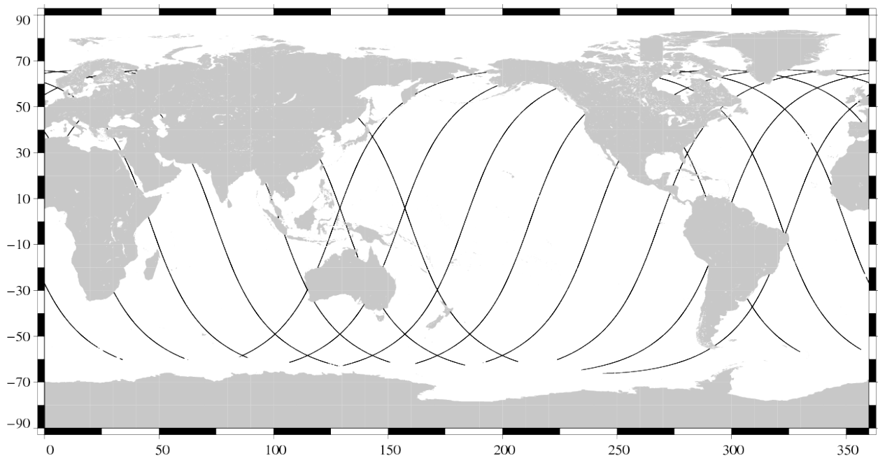
Valid data Jason-1 Cycle 284 (25/09/2009 / 26/09/2009)
