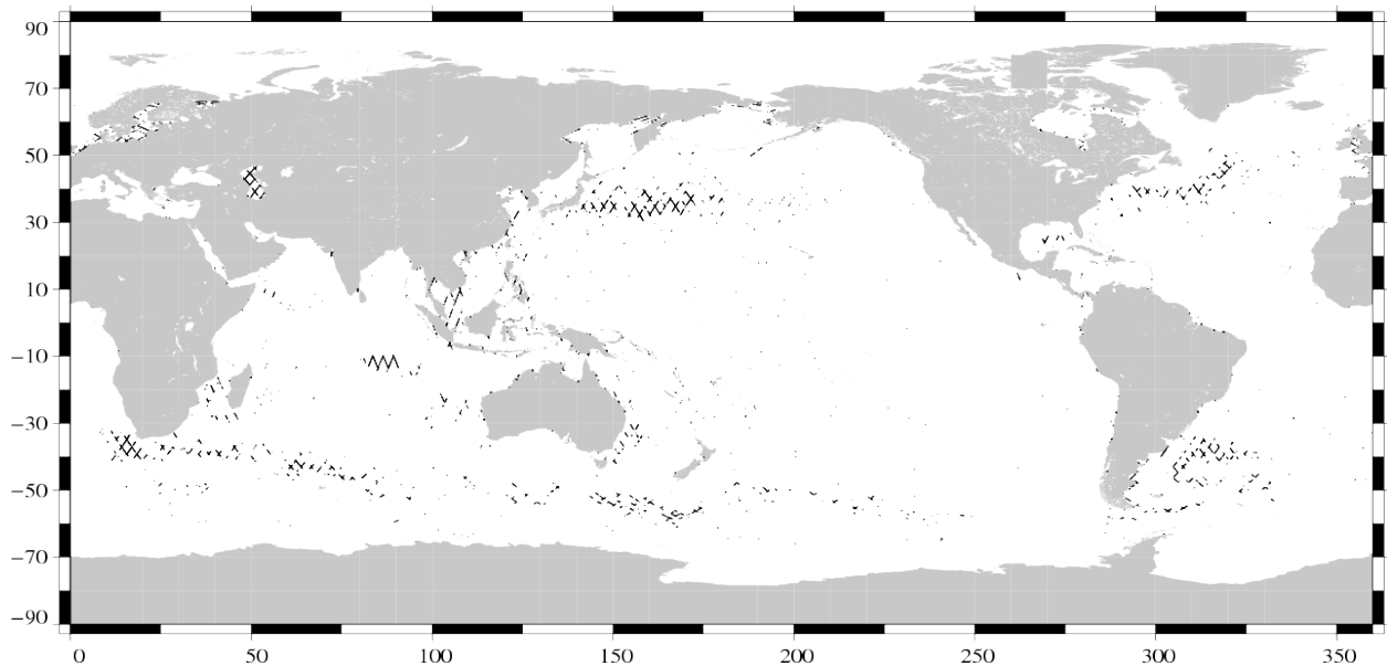
Valid data: (SSH – MSS) differences greater than 30 cm Jason-1 Cycle 290 (14/11/2009 / 24/11/2009)
