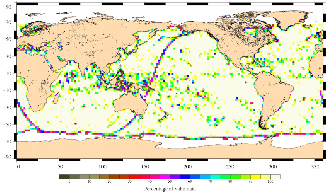
Percentage of valid data relative to the nominal pass Jason-1 Cycle 290 (14/11/2009 / 24/11/2009)
