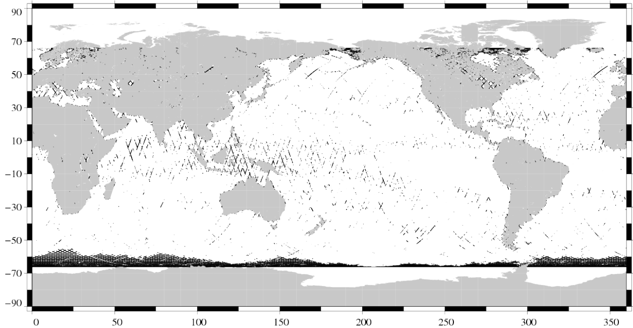
Valid data Jason-1 Cycle 290 (14/11/2009 / 24/11/2009)
