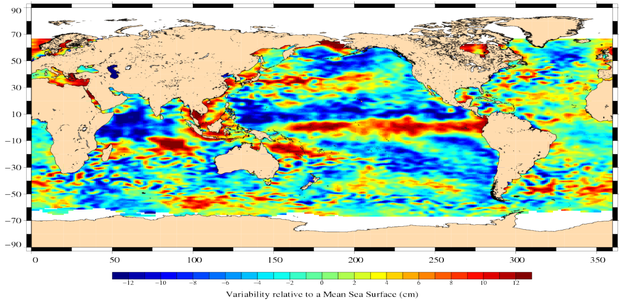
Jason-1 Cycle 292 04/12/2009 – 14/12/2009
