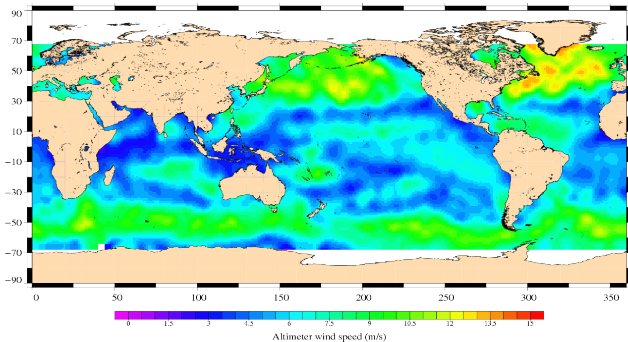
Jason-1 Cycle 292 04/12/2009 - 14/12/2009
