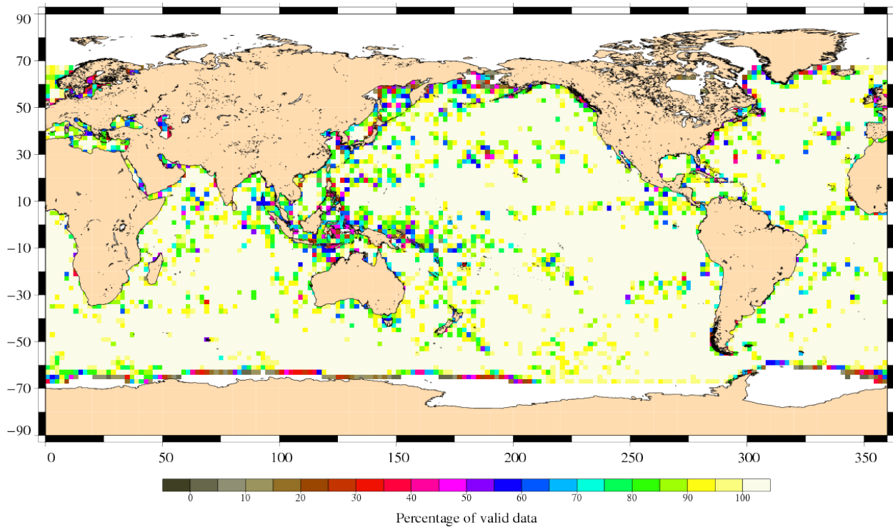
Percentage of valid data relative to the nominal pass Jason-1 Cycle 308 (12/05/2010 / 22/05/2010)
