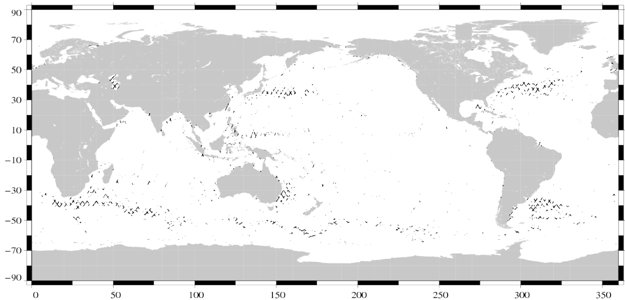
Valid data: (SSH – MSS) differences greater than 30 cm Jason-1 Cycle 308 (12/05/2010 / 22/05/2010)
