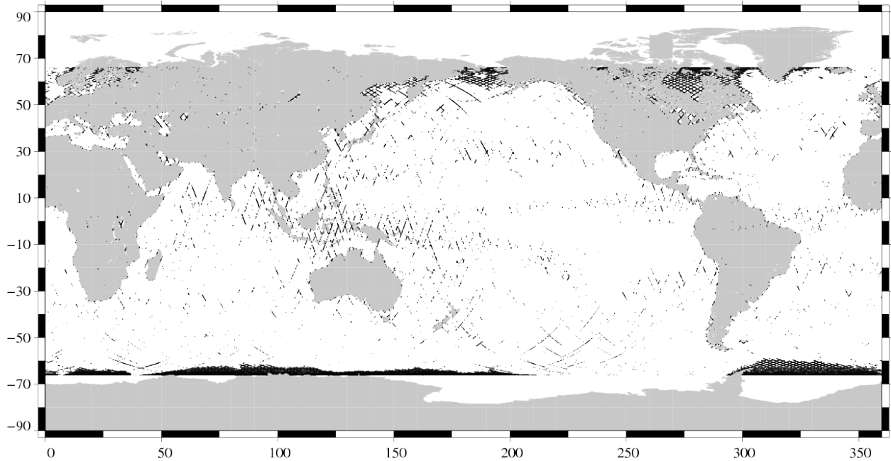
Valid data Jason-1 Cycle 308 (12/05/2010 / 22/05/2010)
