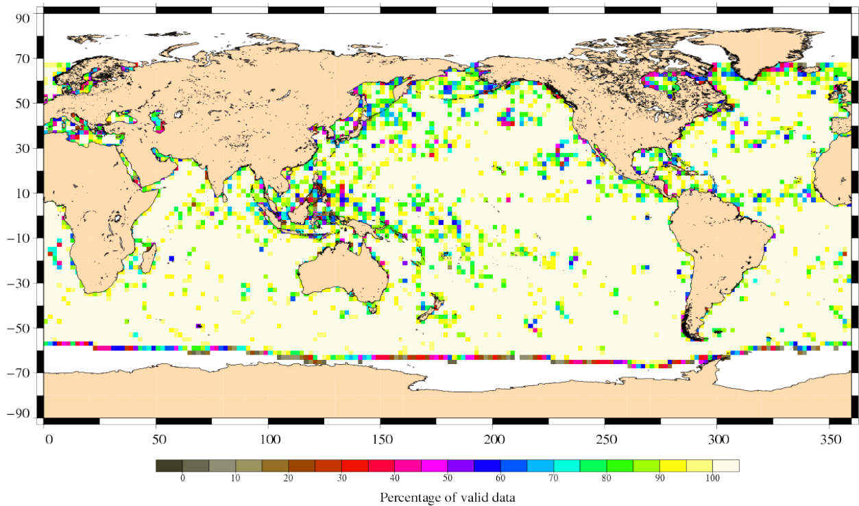
Percentage of valid data relative to the nominal pass Jason-1 Cycle 314 (10/07/2010 / 20/07/2010)
