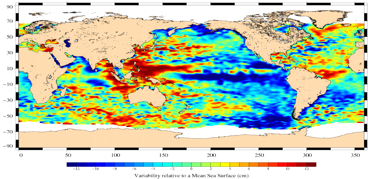
Jason-1 Cycle 318 19/08/2010 – 29/08/2010
