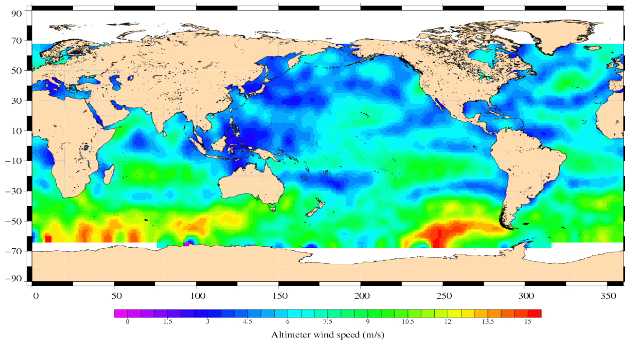
Jason-1 Cycle 318 19/08/2010 – 29/08/2010
