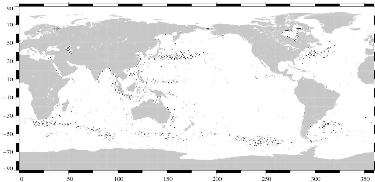
Valid data: (SSH – MSS) differences greater than 30 cm Jason-1 Cycle 323 (08/10/2010 / 18/10/2010)
