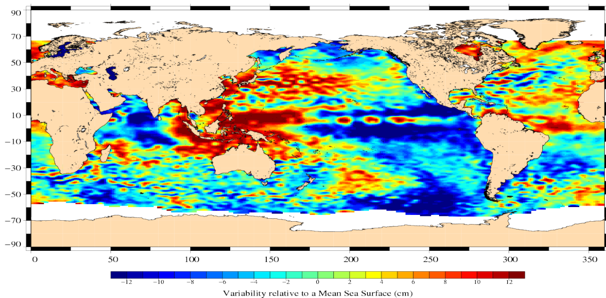
Jason-1 Cycle 323 08/10/2010 – 18/10/2010
