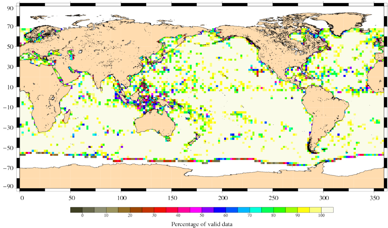
Percentage of valid data relative to the nominal pass Jason-1 Cycle 323 (08/10/2010 / 18/10/2010)
