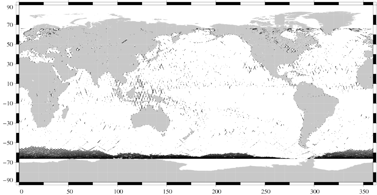
Valid data Jason-1 Cycle 323 (08/10/2010 / 18/10/2010)
