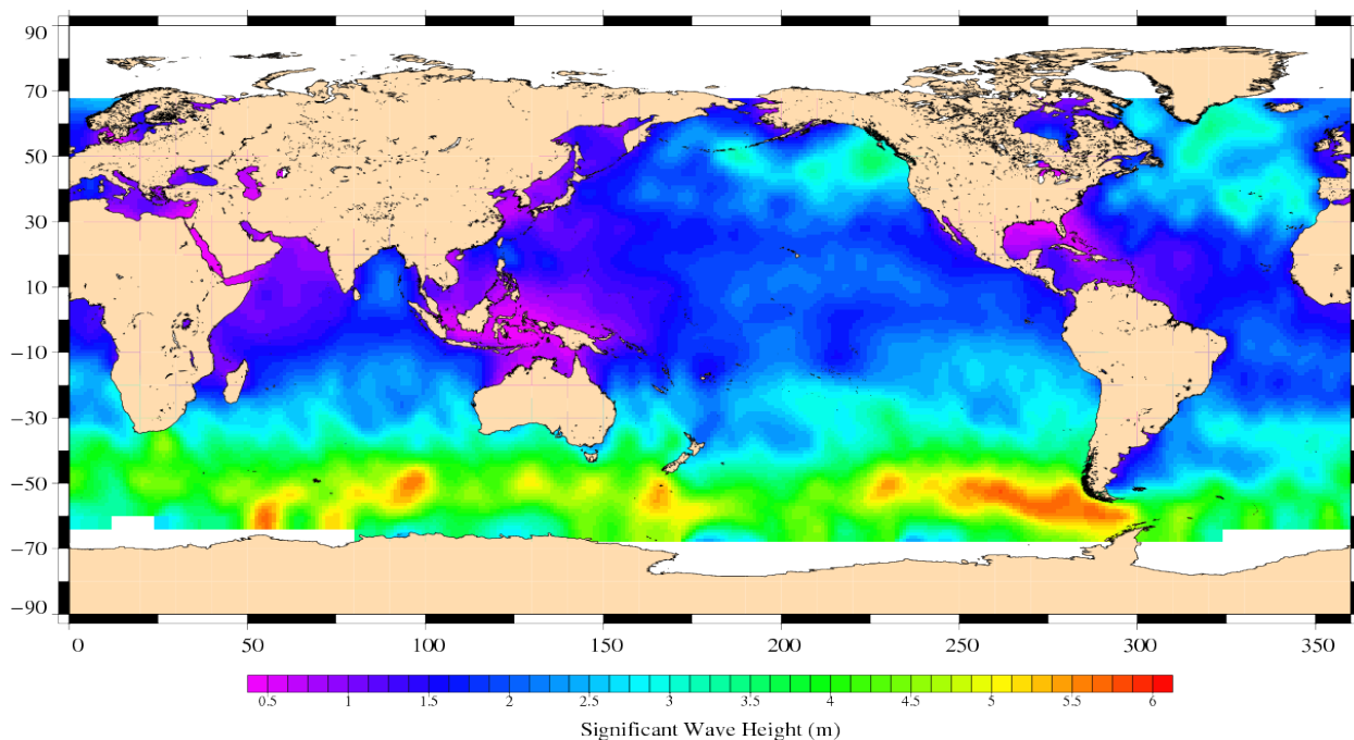
Jason-1 Cycle 323 08/10/2010 - 18/10/2010
