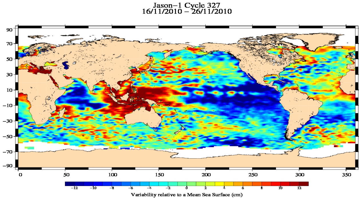
Valid data: (SSH – MSS) differences greater than 30 cm Jason-1 Cycle 327 (16/11/2010 / 26/11/2010)
