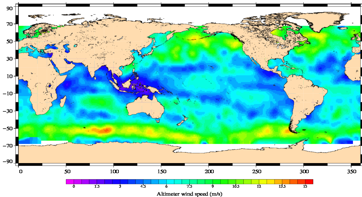
Jason-1 Cycle 327 16/11/2010 – 26/11/2010
