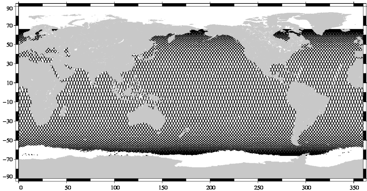
Valid data Jason-1 Cycle 327 (16/11/2010 / 26/11/2010)
