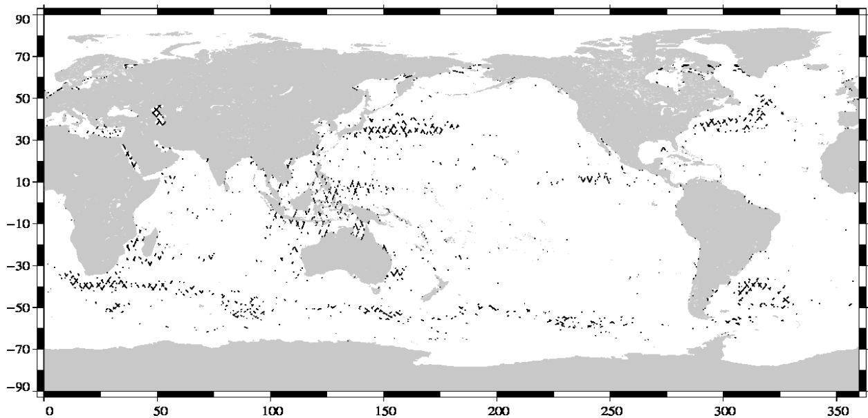
Valid data: (SSH – MSS) differences greater than 30 cm Jason-1 Cycle 327 (16/11/2010 / 26/11/2010)
