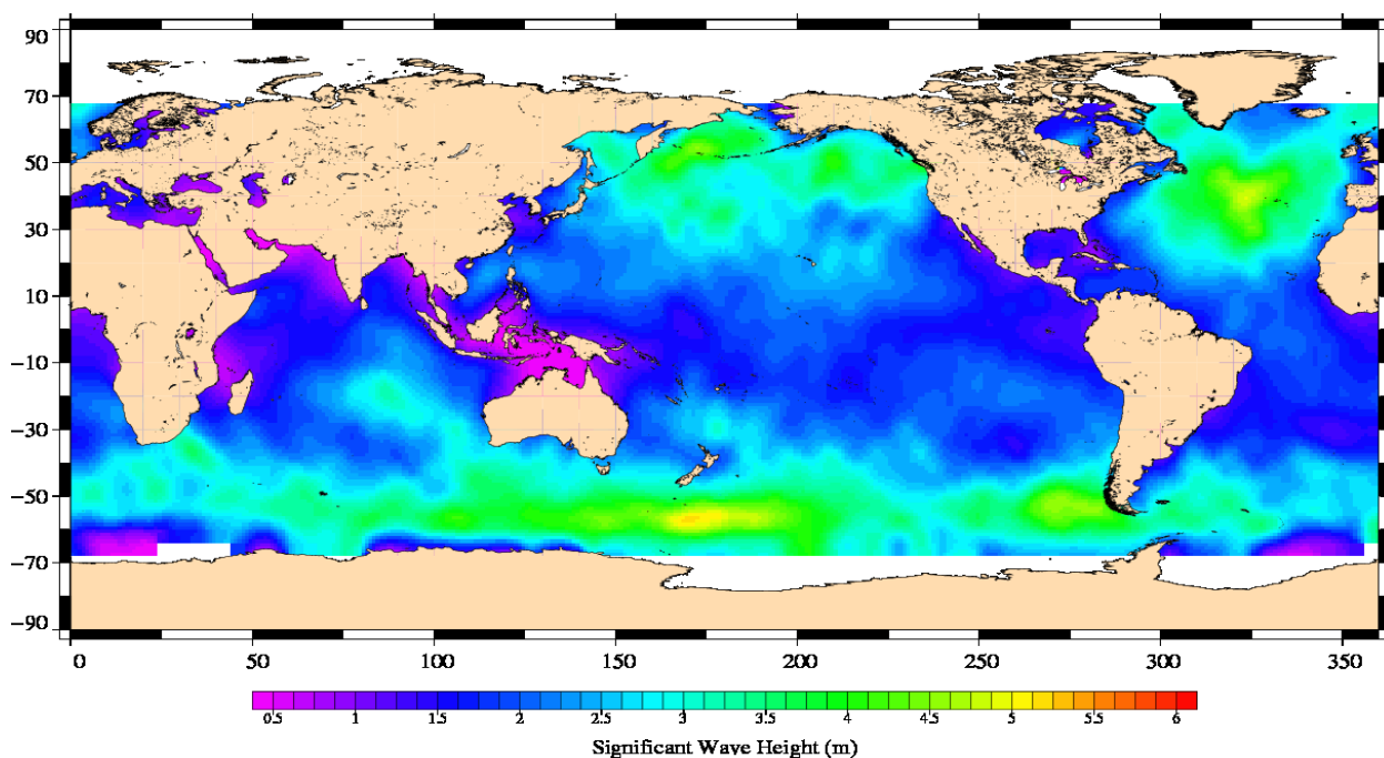
Jason-1 Cycle 328 26/11/2010 - 06/12/2010
