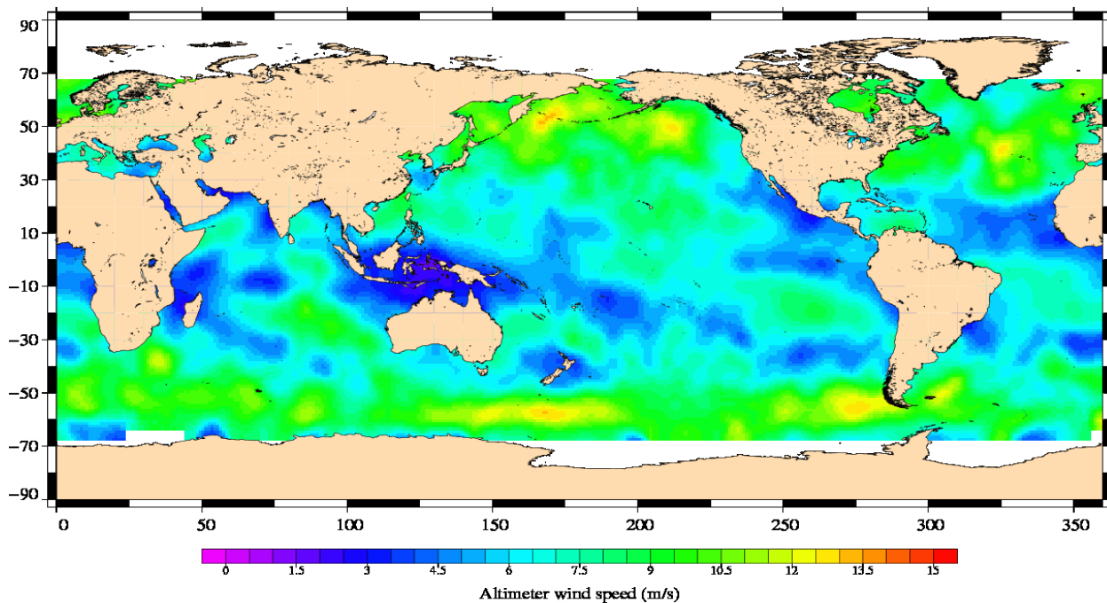
Jason-1 Cycle 328 26/11/2010 - 06/12/2010
