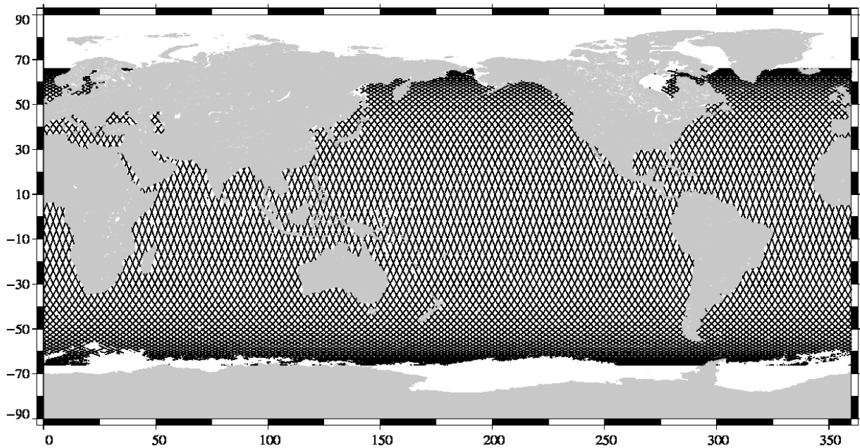
Valid data Jason-1 Cycle 330 (16/12/2010 / 26/12/2010)
