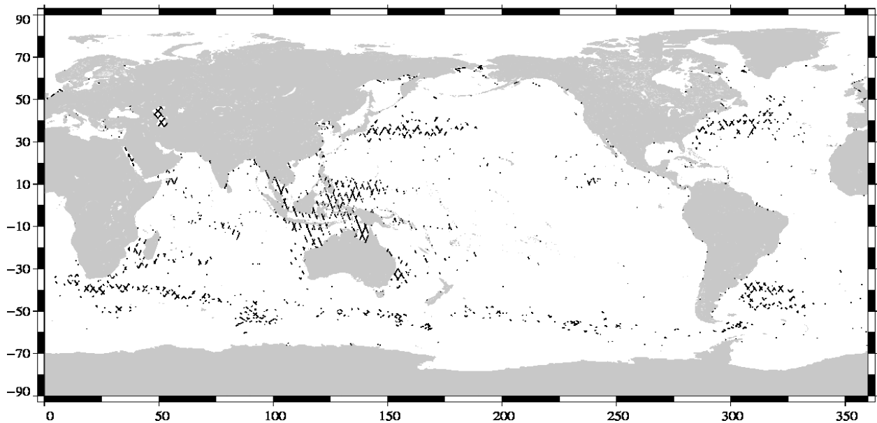
Valid data: (SSH – MSS) differences greater than 30 cm Jason-1 Cycle 330 (16/12/2010 / 26/12/2010)
