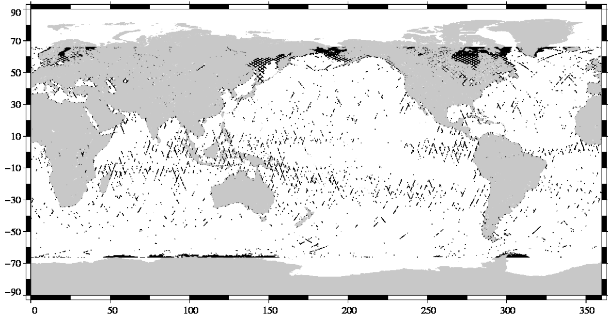
Valid data Jason-1 Cycle 337 (23/02/2011 / 05/03/2011)
