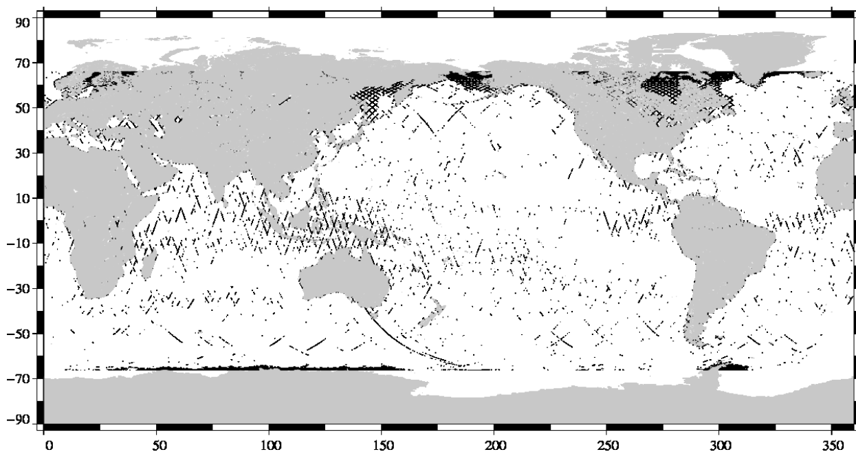
Edited measurements Jason-1 Cycle 339 (15/03/2011 / 25/03/2011)
