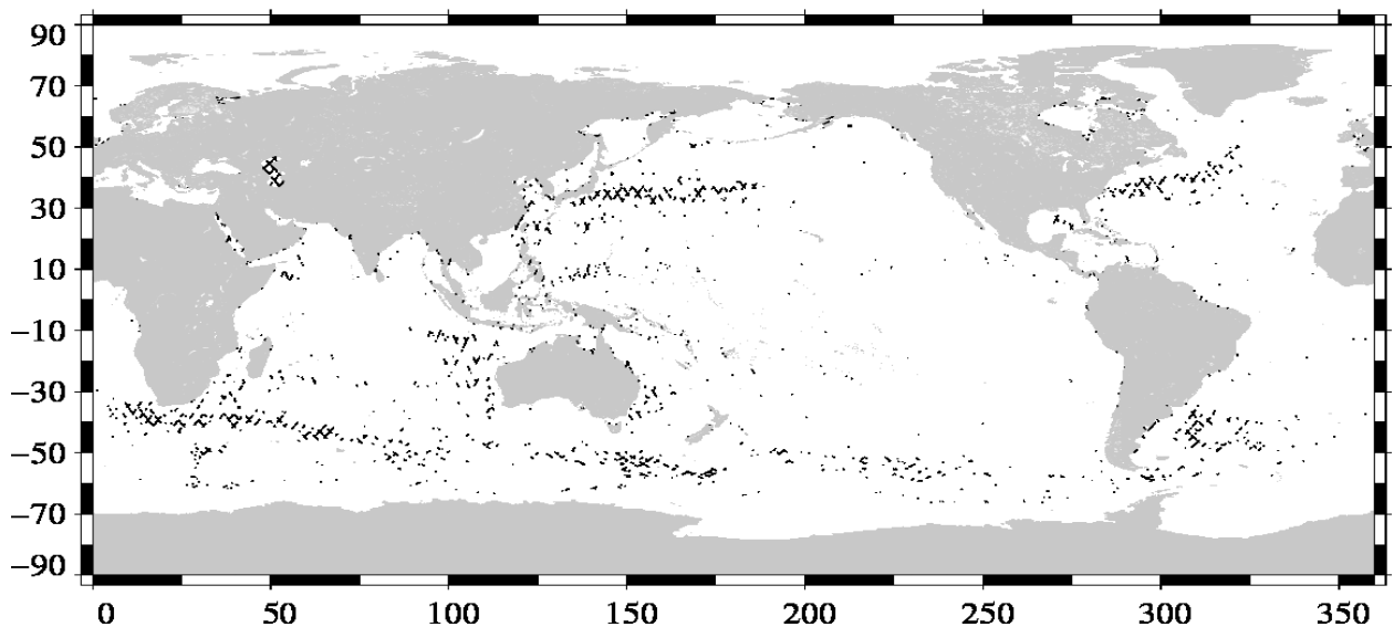
Valid data: (SSH – MSS) differences greater than 30 cm Jason-1 Cycle 354 (11/08/2011 / 21/08/2011)
