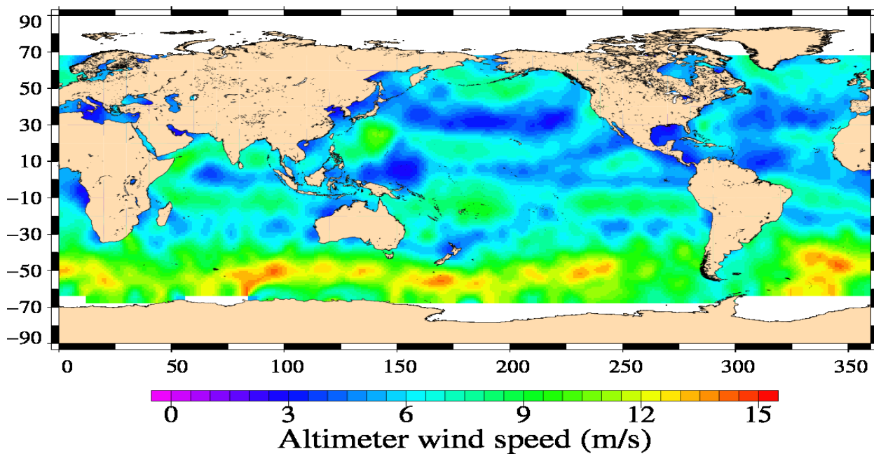
Jason-1 Cycle 355 21/08/2011 – 31/08/2011
