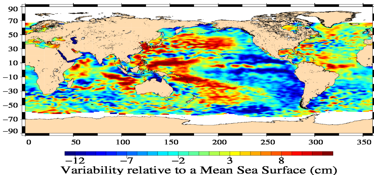
Jason-1 Cycle 355 21/08/2011 – 31/08/2011
