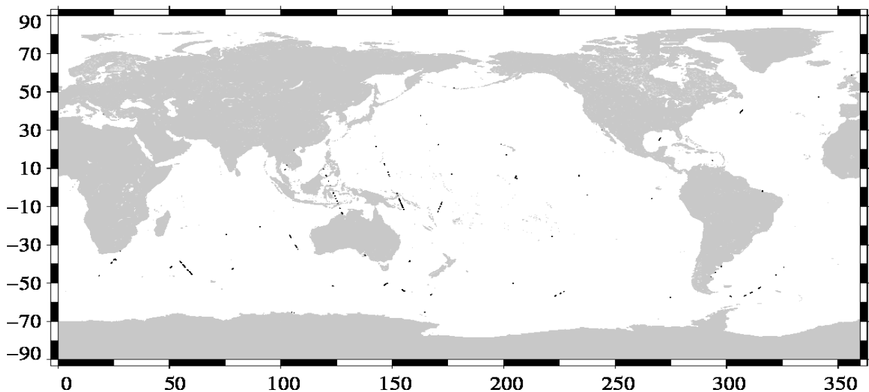
Valid data: (SSH – MSS) differences greater than 30 cm Jason-1 Cycle 373 (15/02/2012 / 16/02/2012)
