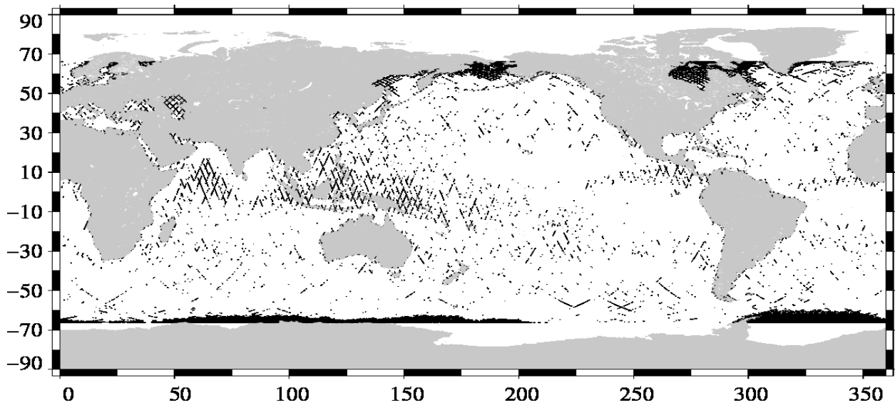
Valid data Jason-1 Cycle 500 (07/05/2012 / 18/05/2012)
