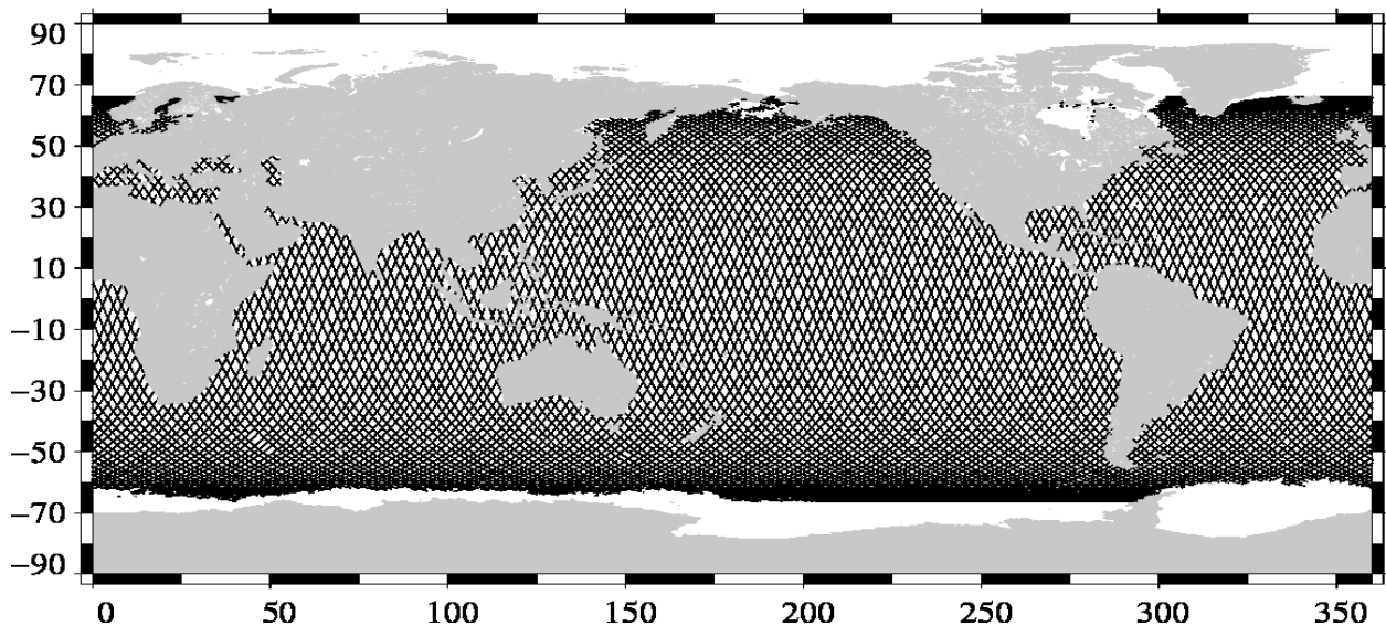
Valid data Jason-1 Cycle 502 (29/05/2012 / 09/06/2012)
