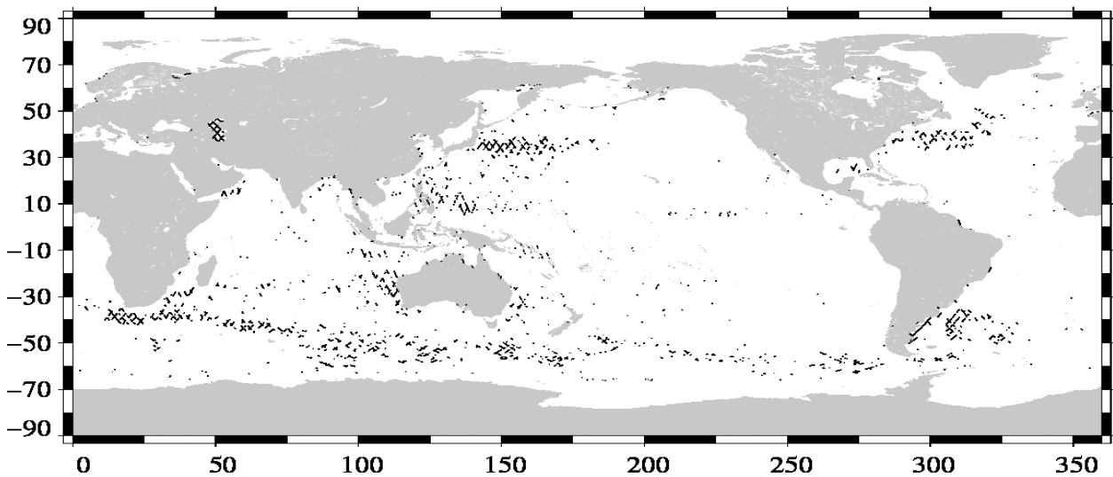
Valid data: (SSH – MSS) differences greater than 30 cm Jason-1 Cycle 502 (29/05/2012 / 09/06/2012)
