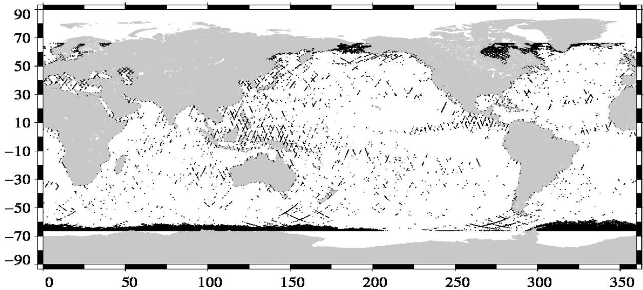
Edited measurements Jason-1 Cycle 502 (29/05/2012 / 09/06/2012)
