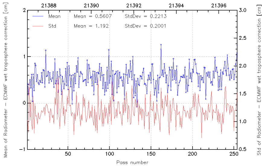
FIG. 11 – Pass monitoring of wet troposphere differences between radiometer and ECMWF model for Jason-2 cycle 002.
