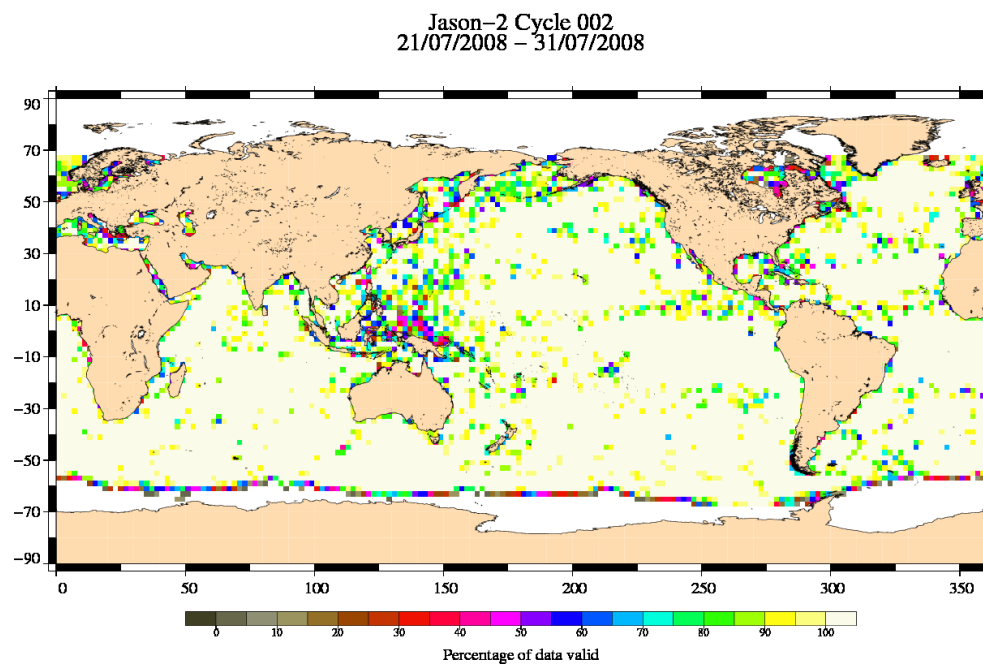
FIG. 3 – Percentage of valid measurements for cycle 002.
