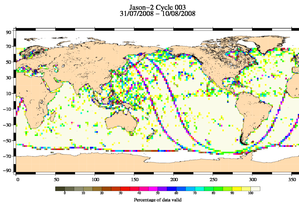
FIG. 3 – Percentage of valid measurements for cycle 003.
