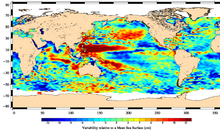
FIG. 18 – Sea level anomaly relative to MSS for cycle 003.
