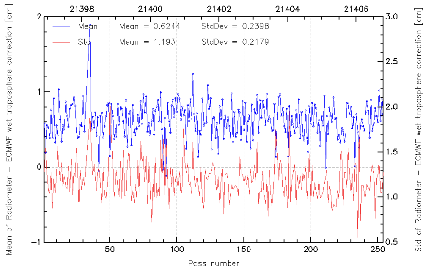
FIG. 11 – Pass monitoring of wet troposphere differences between radiometer and ECMWF model for Jason-2 cycle 003.
