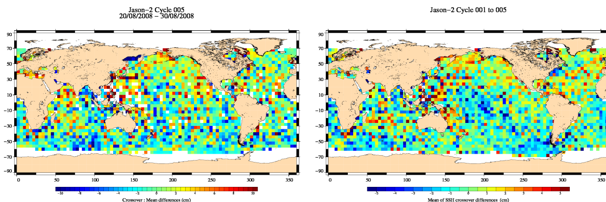
FIG. 13 – Mean SSH at crossovers for cycle 005 (left) and over the whole Jason-2 period (right).
