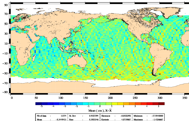
FIG. 20 – Jason-1 – Jason-2 SLA differences (without corrections) for cycle 005.
