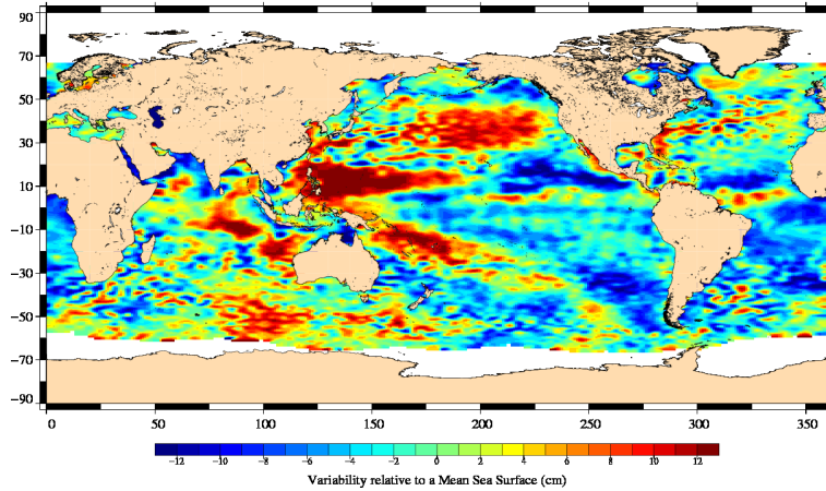
FIG. 18 – Sea level anomaly relative to MSS for cycle 005.
