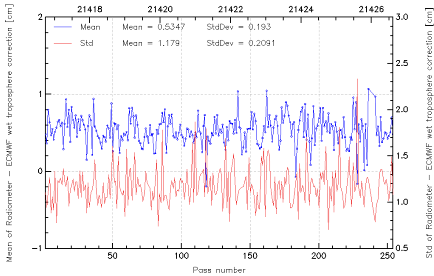
FIG. 11 – Pass monitoring of wet troposphere differences between radiometer and ECMWF model for Jason-2 cycle 005.
